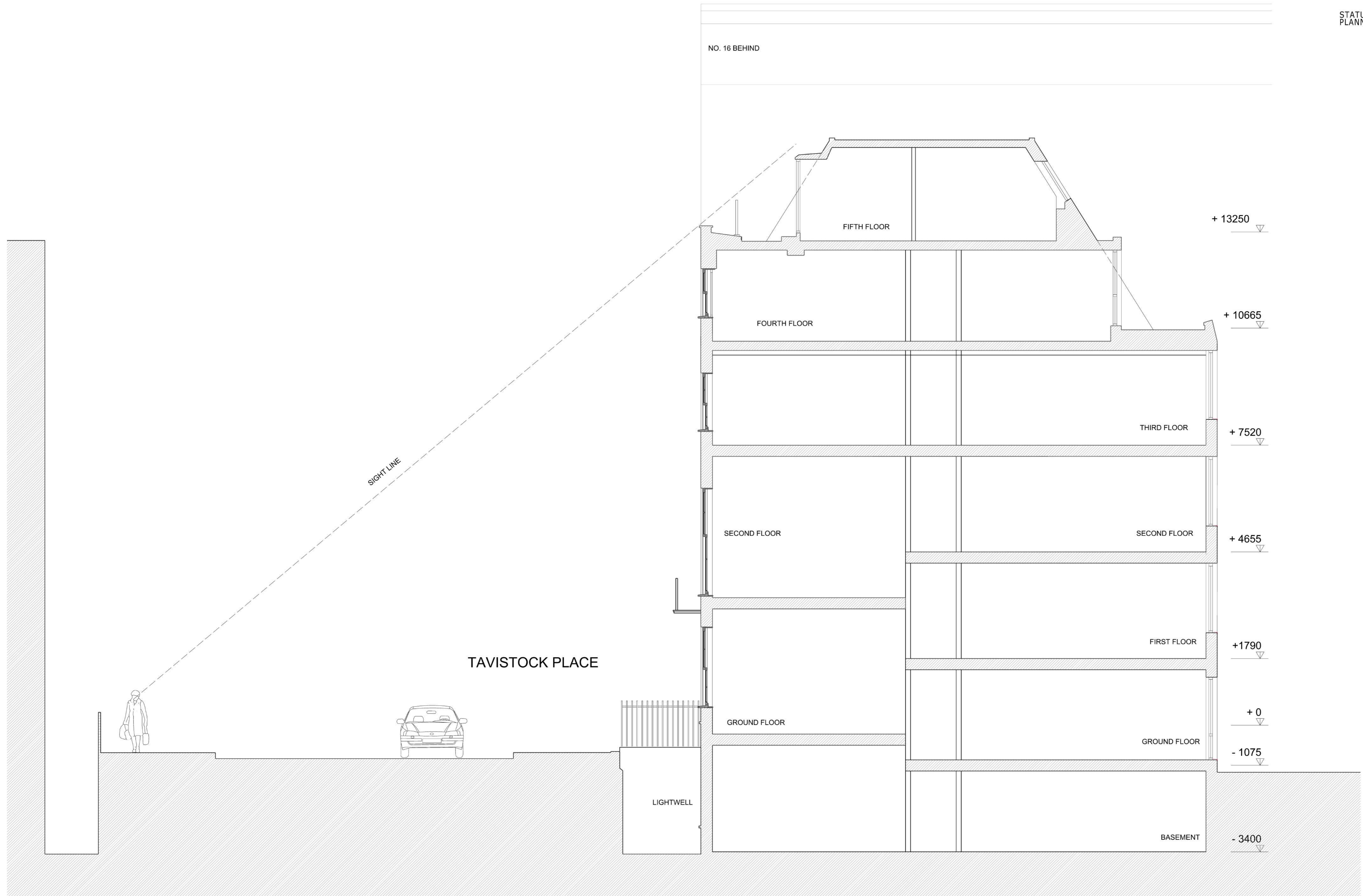
INDICATIVE SECTION
