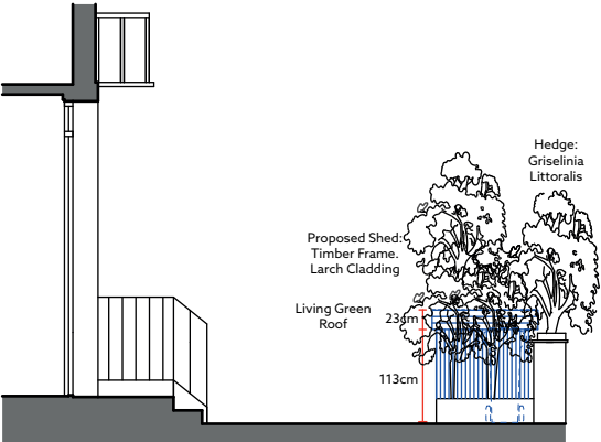
85 PROPOSED SECTION AA
