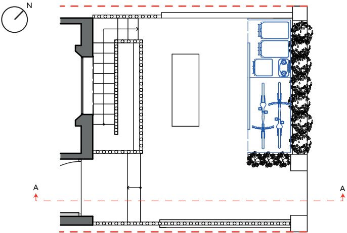
85 PROPOSED FRONT GARDEN PLAN
