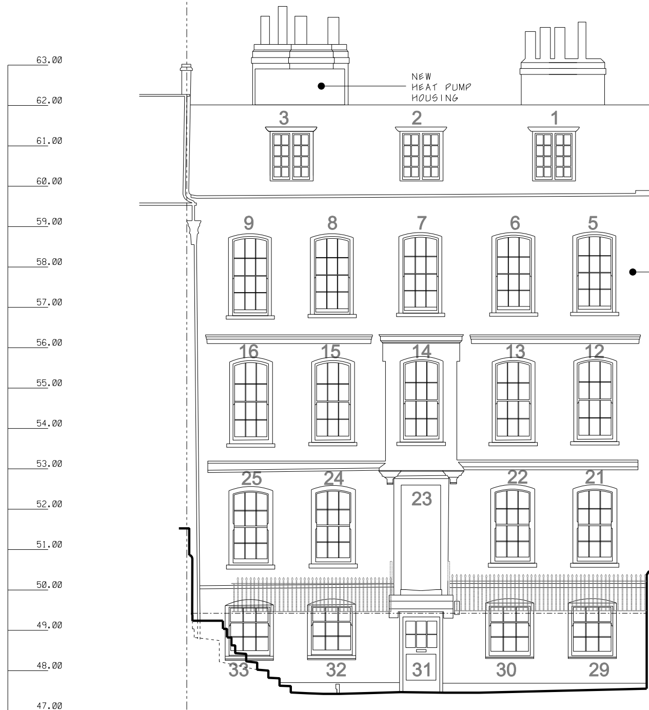
Front elevation
