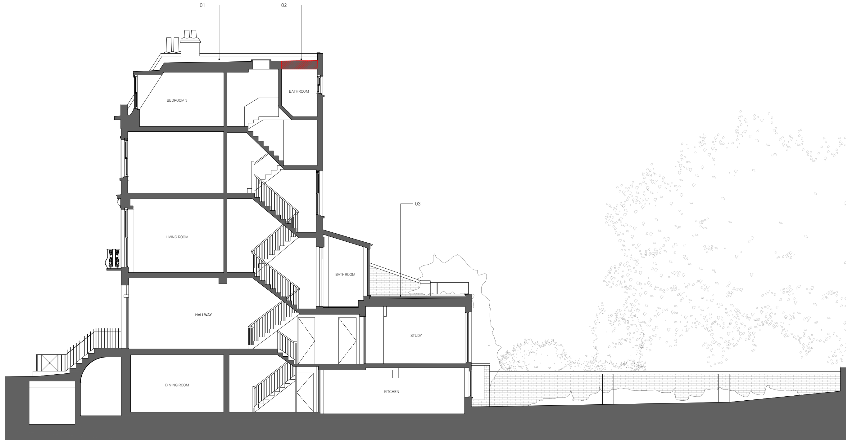
EXISTING SECTION AA 1:100
