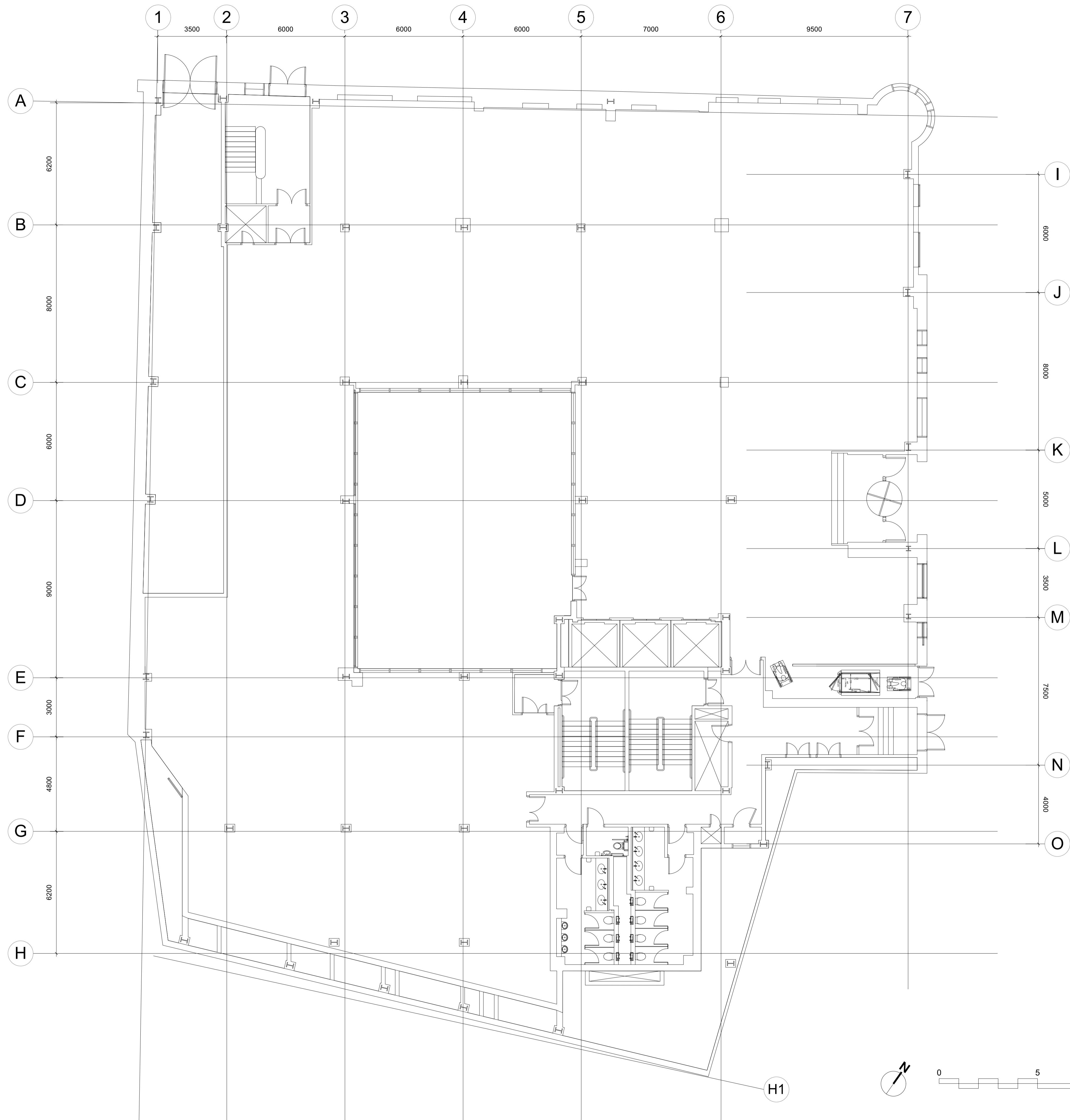
1 Ground Floor Plan, Existing 4677-ST-EX-02-100 Scale: 1:100
