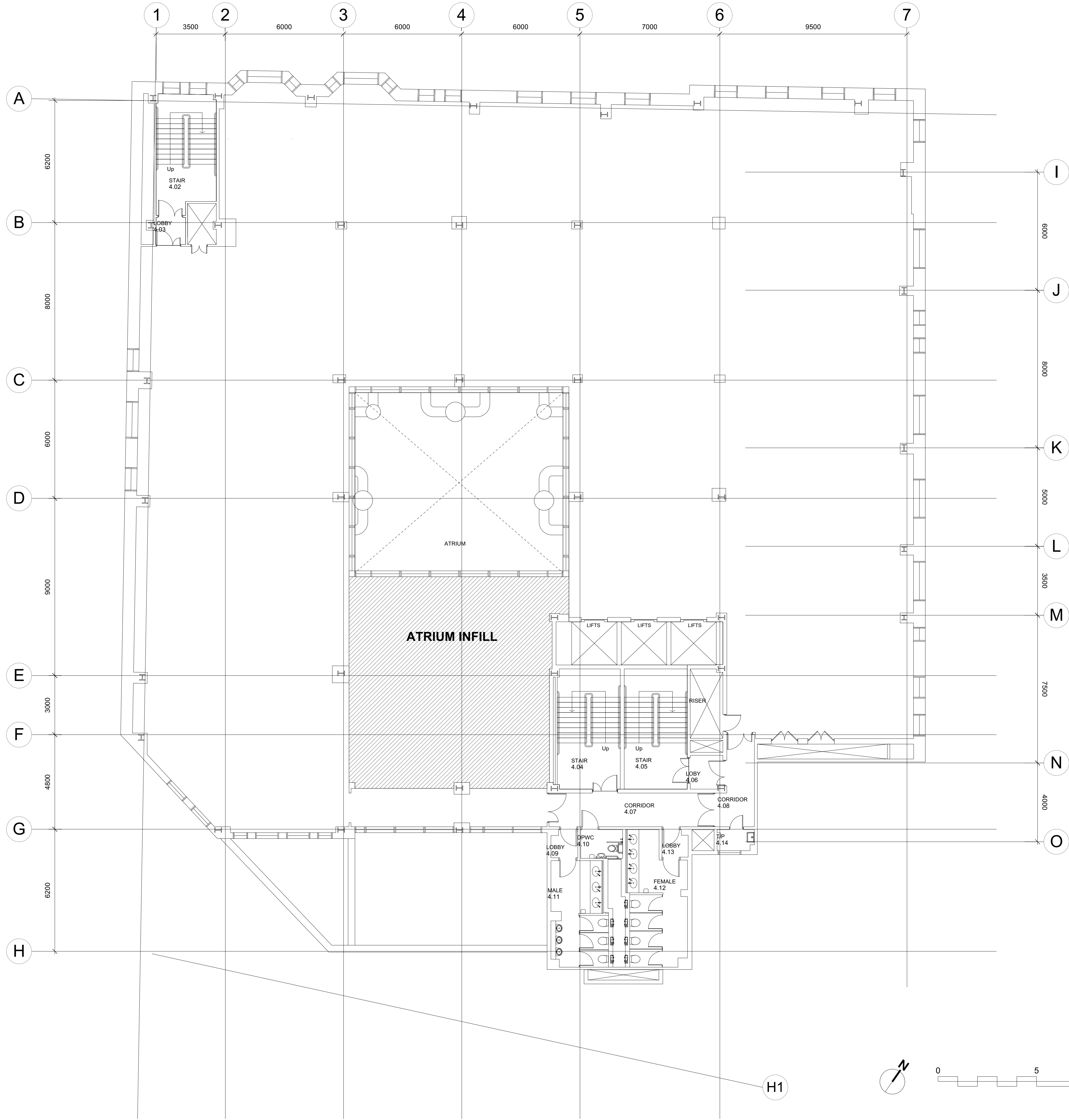
1 Fourth Floor Plan, Proposed 4677-ST-PR-02-104 Scale: 1:100
