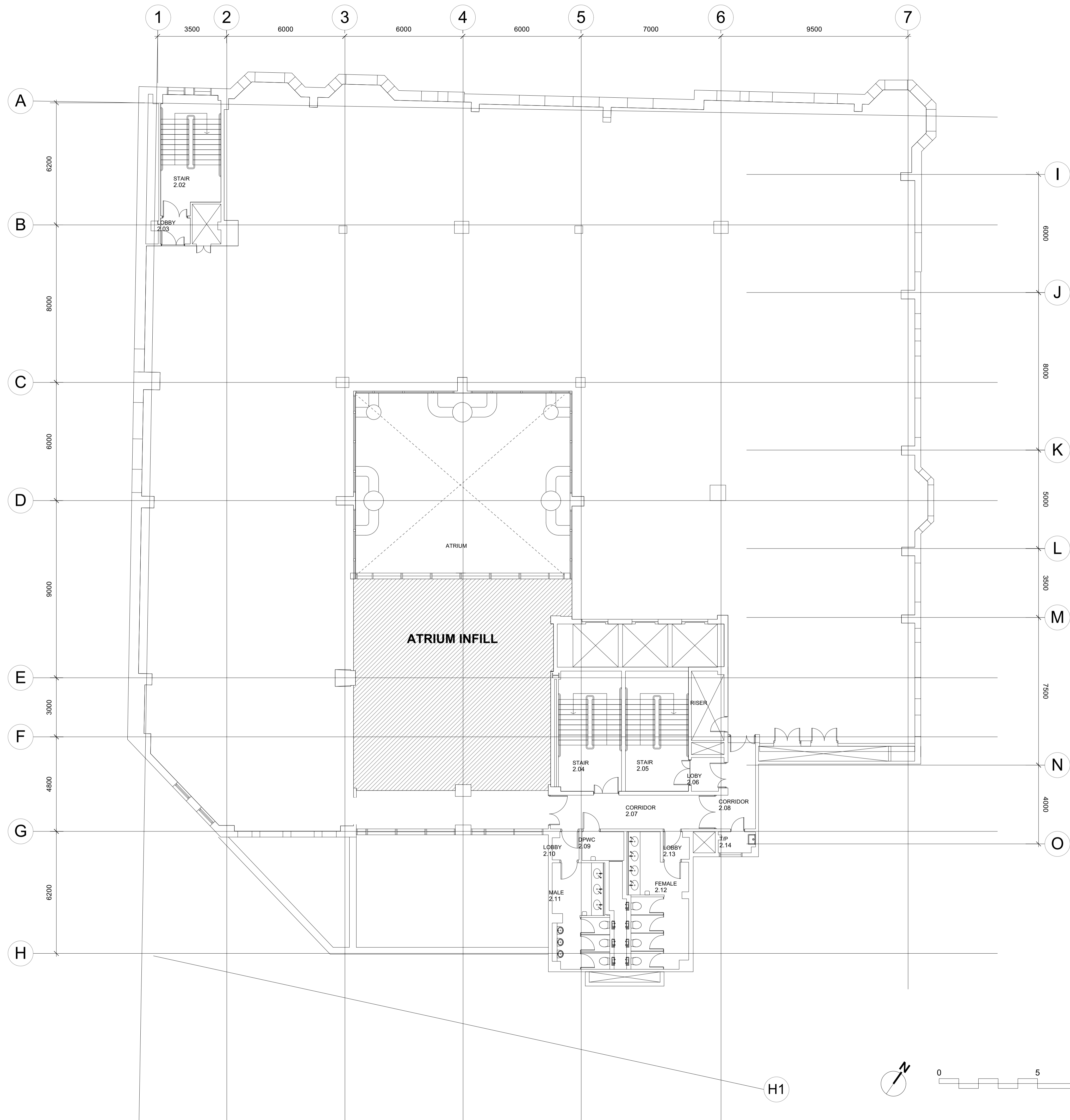
1 Second Floor Plan, Proposed 4677-ST-PR-02-102 Scale: 1:100
