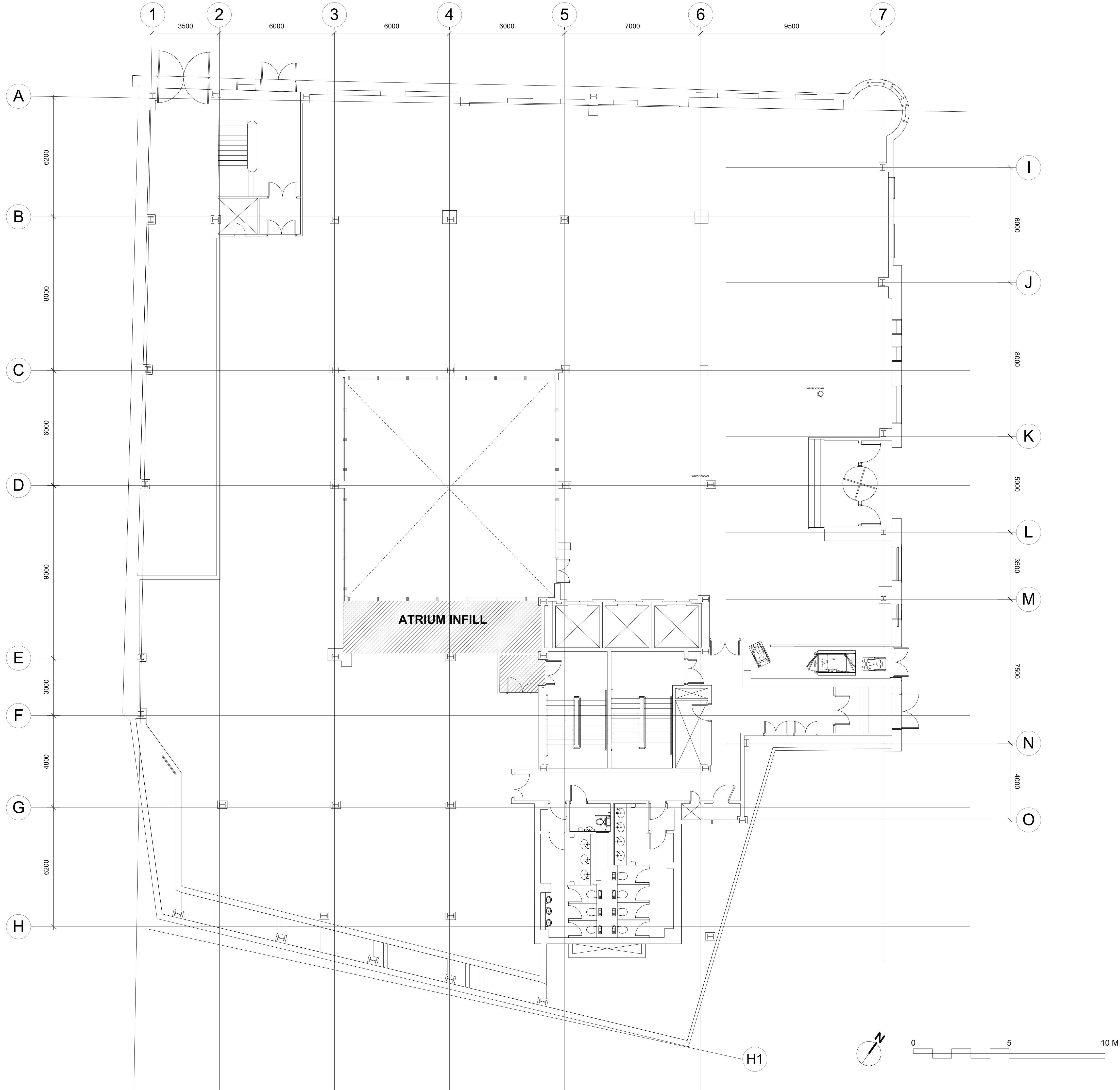
1 Ground Floor Plan, Proposed 4677-ST-PR-02-100 Scale: 1:100
