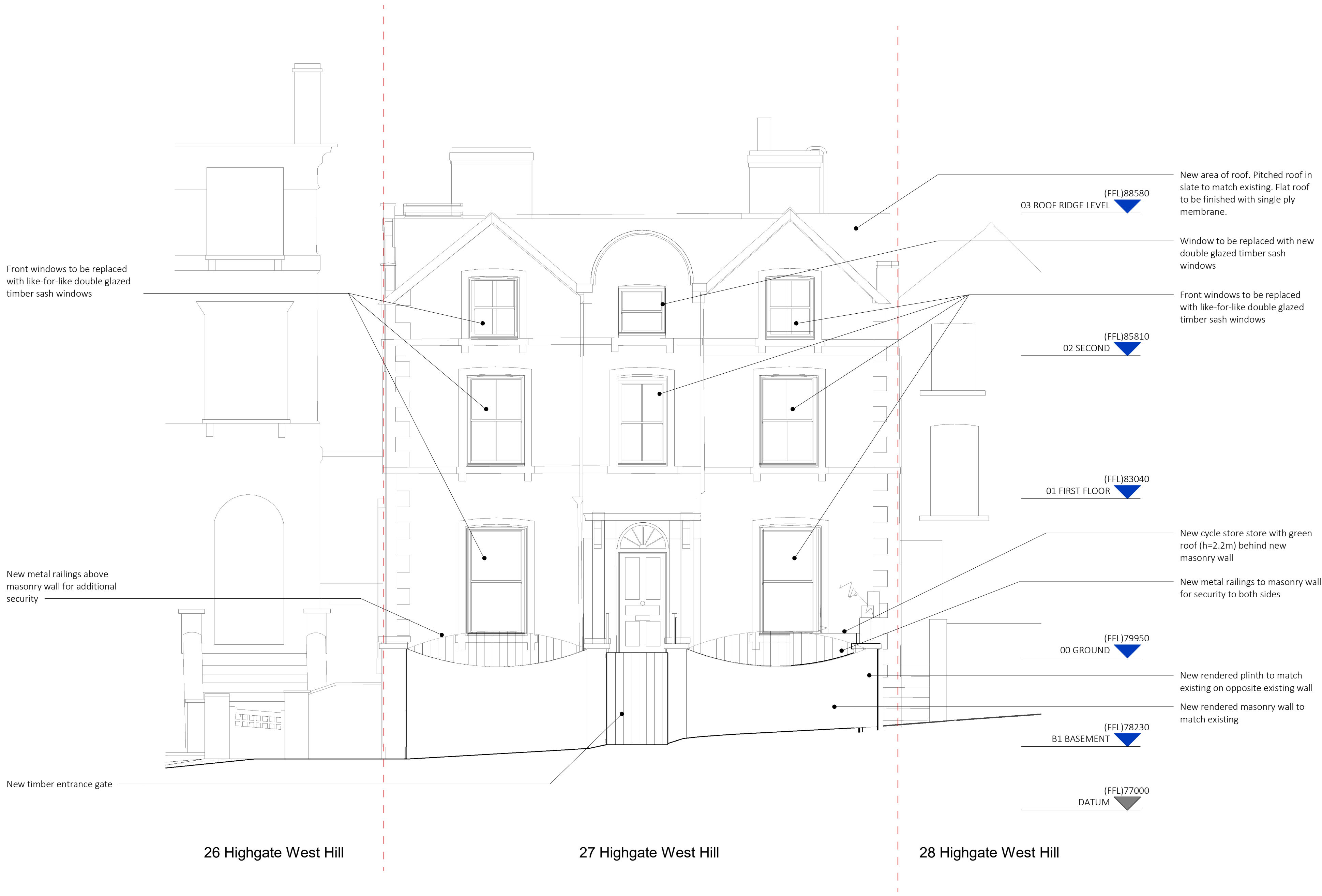
1 1 : 50 PROPOSED FRONT ELEVATION
