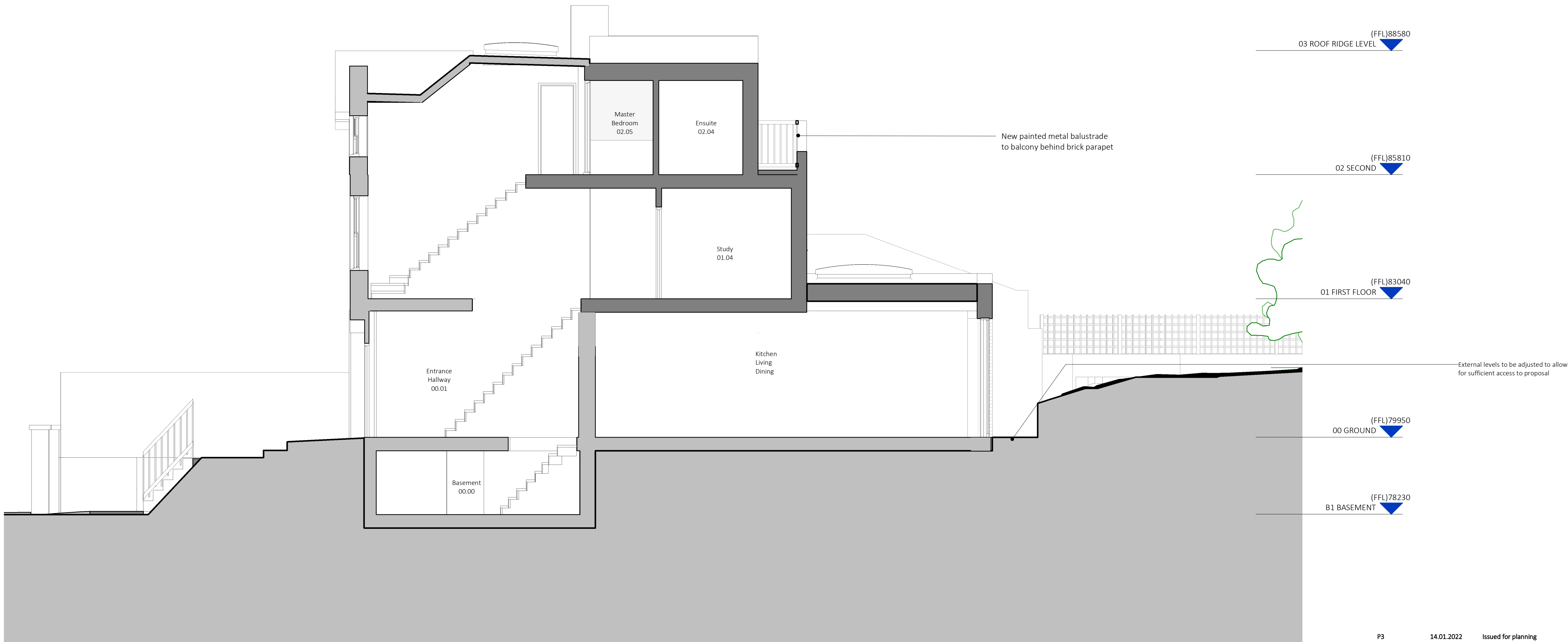
1 1 : 50 PROPOSED SECTION A-A
