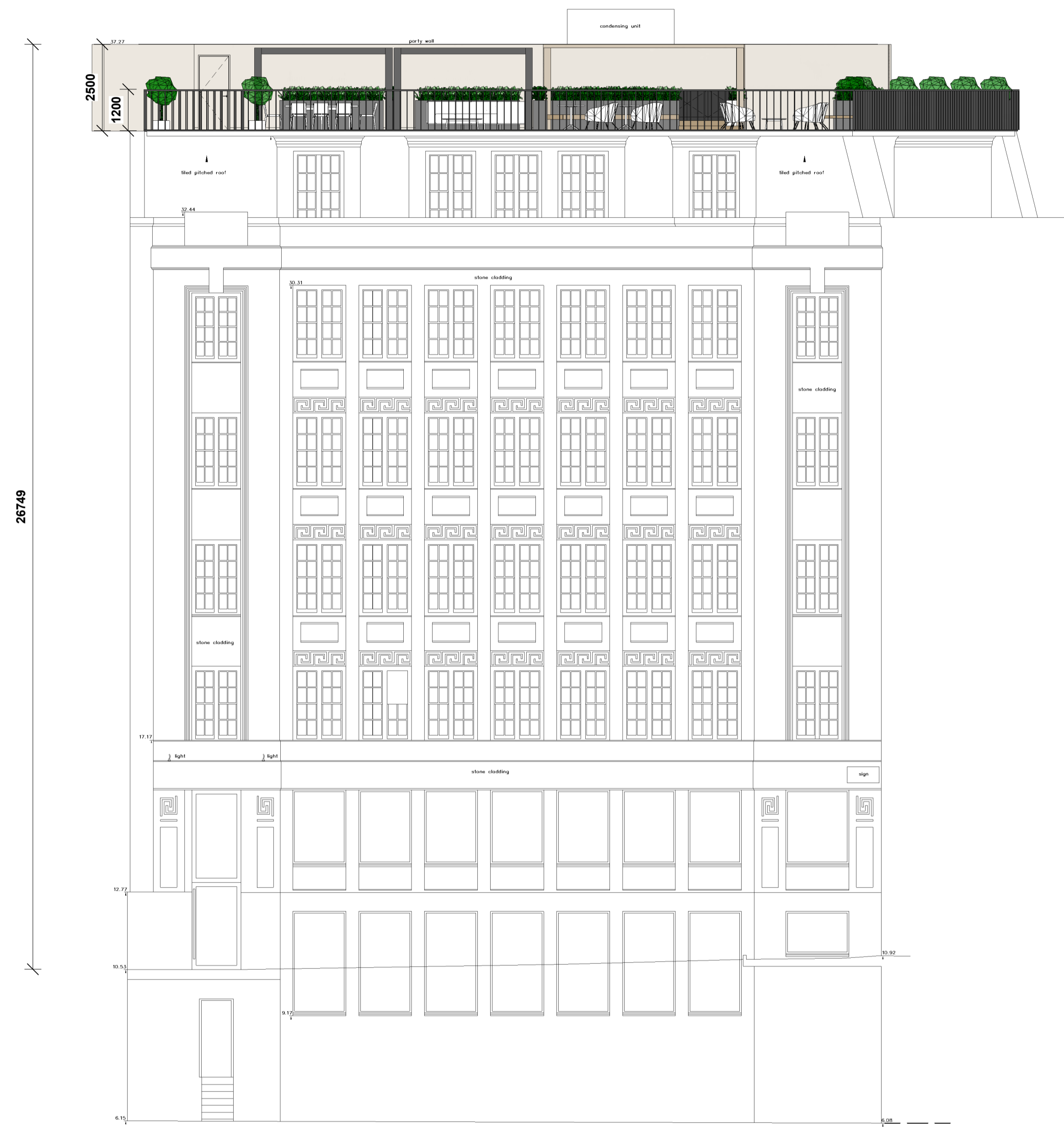
3 Proposed_Farringdon Elevation 1 : 100
