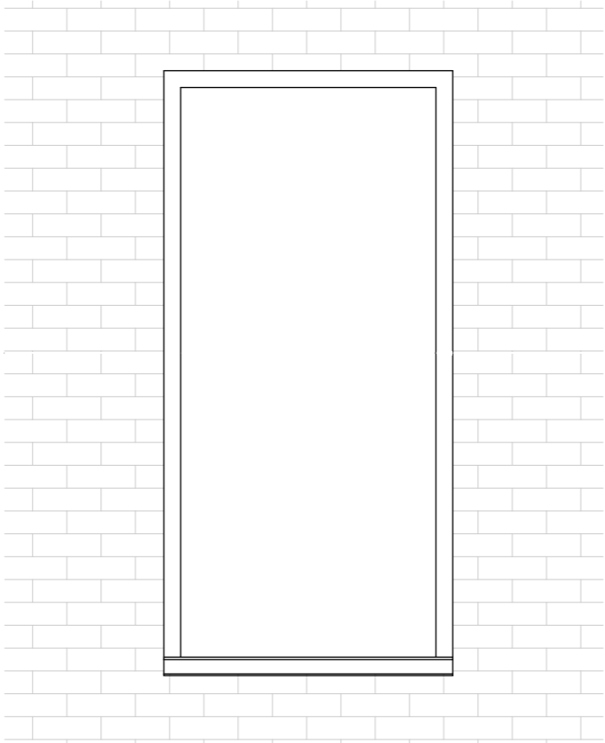
.....Proposed Window Elevation..... 1:20.
