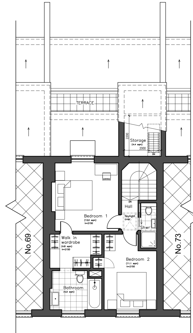
PROPOSED THIRD FLOOR PLAN
