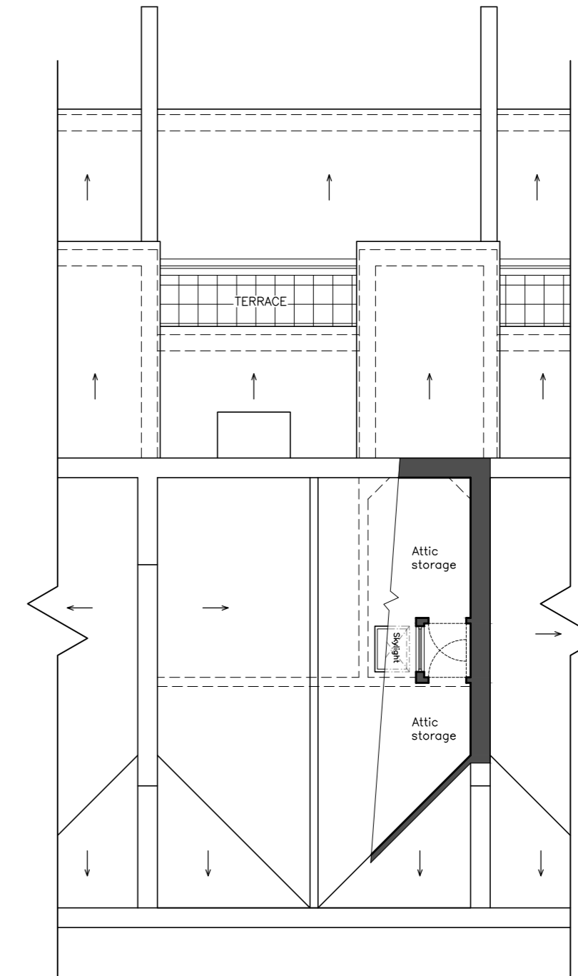
PROPOSED ATTIC FLOOR PLAN
