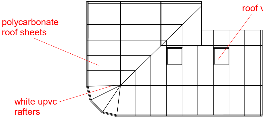
ROOF PLAN
