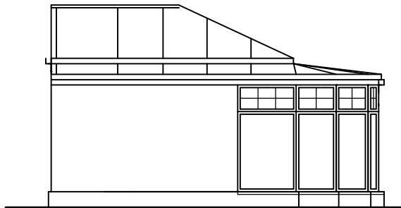
left (south west) elevation
