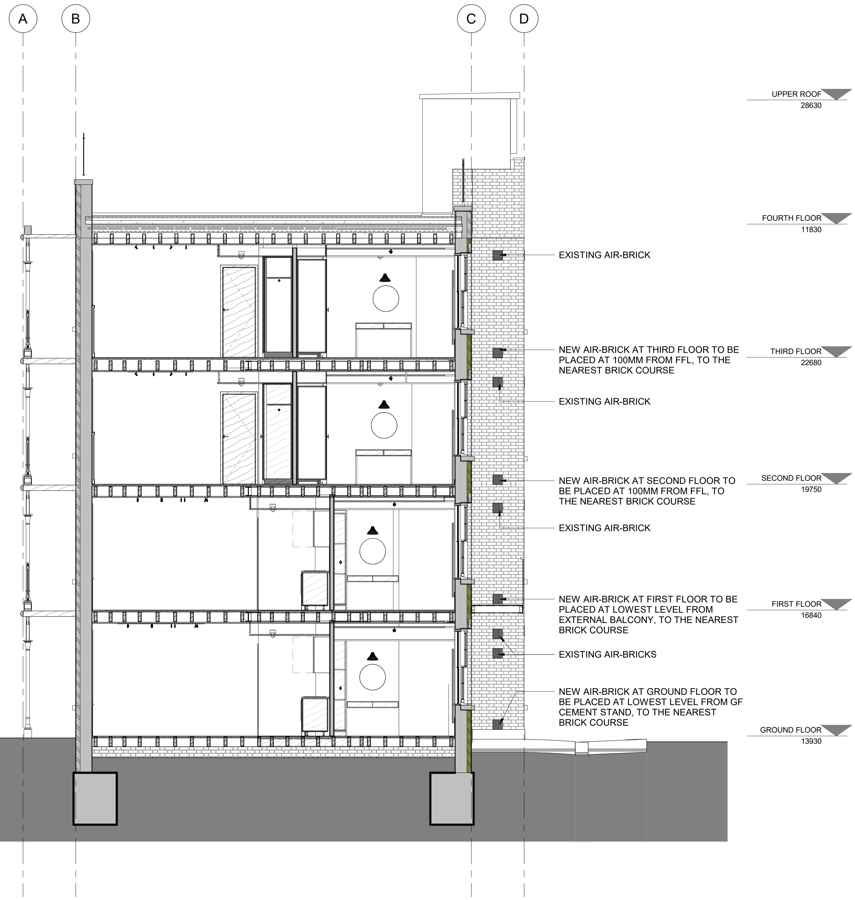
1 07122 PROPOSED - SECTION F 1:50
