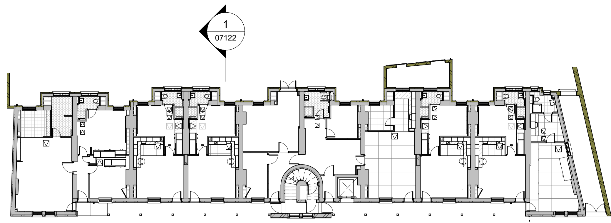
2 07122 KEY PLAN 1:200
