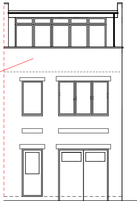
front (south east) elevation
