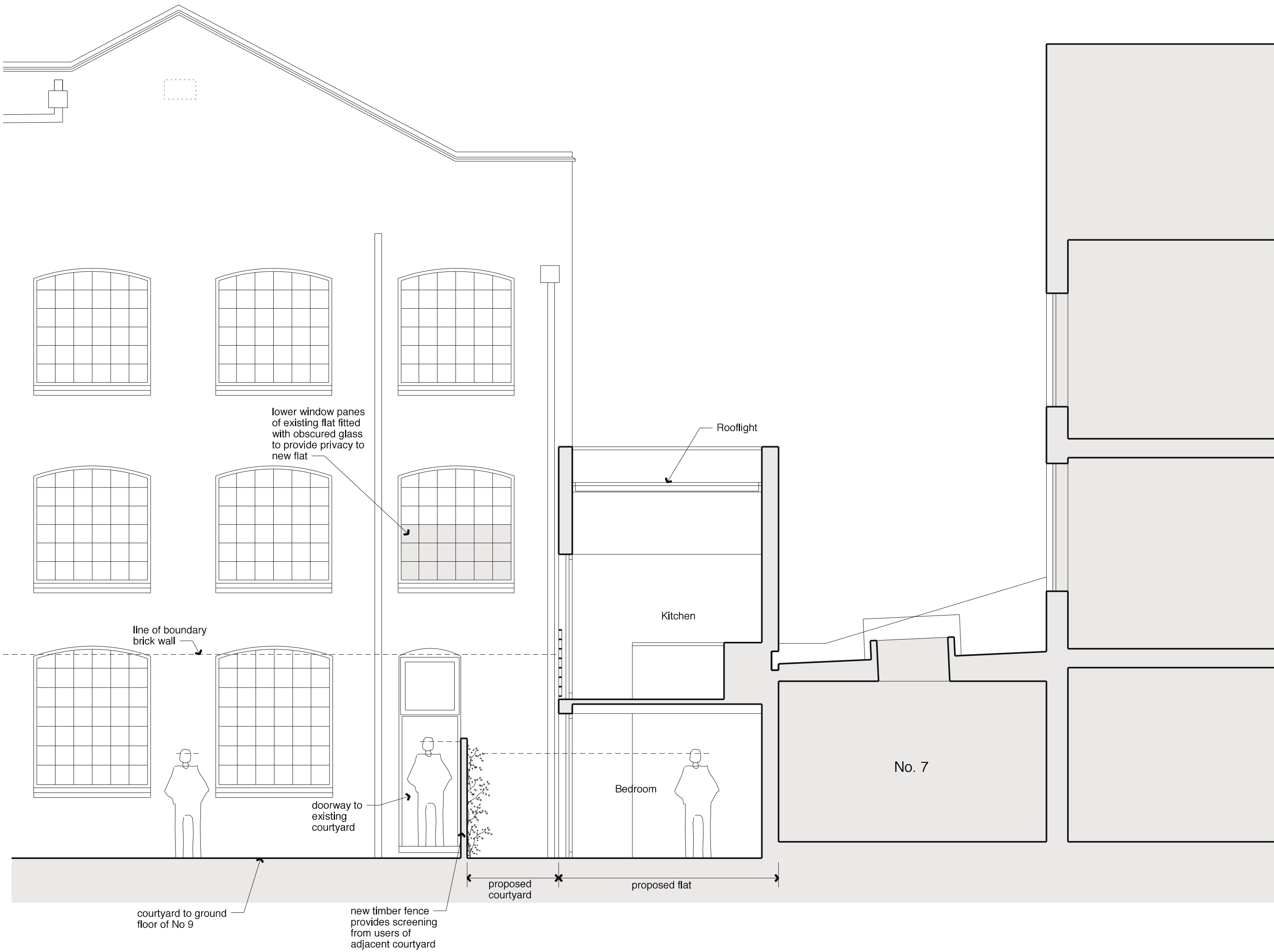
Section CC
