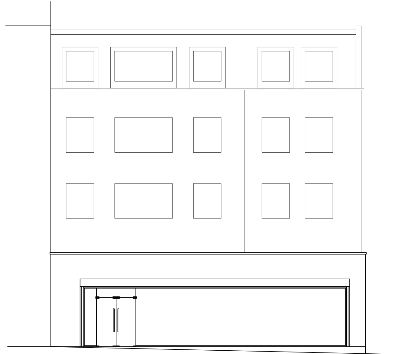
PROPOSED FRONT ELEVATION (shutters up)
