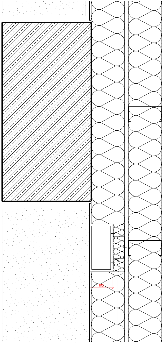
2 Bat Box Plan
