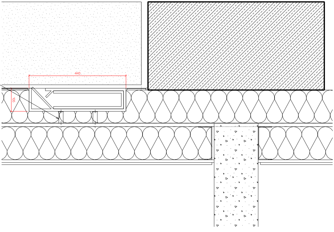
3 Bat Box Section
