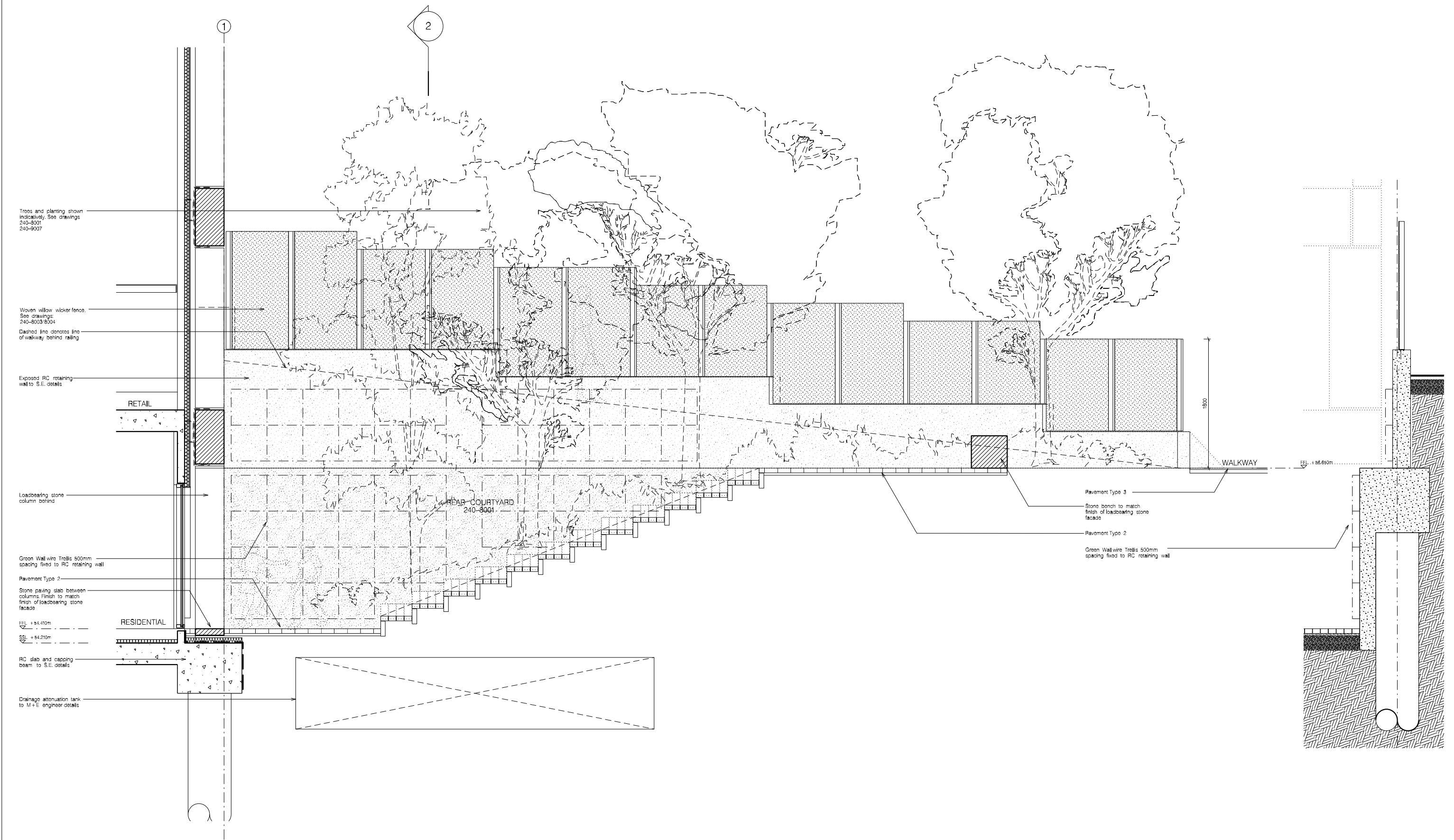
① Proposed Rear Courtyard Section
