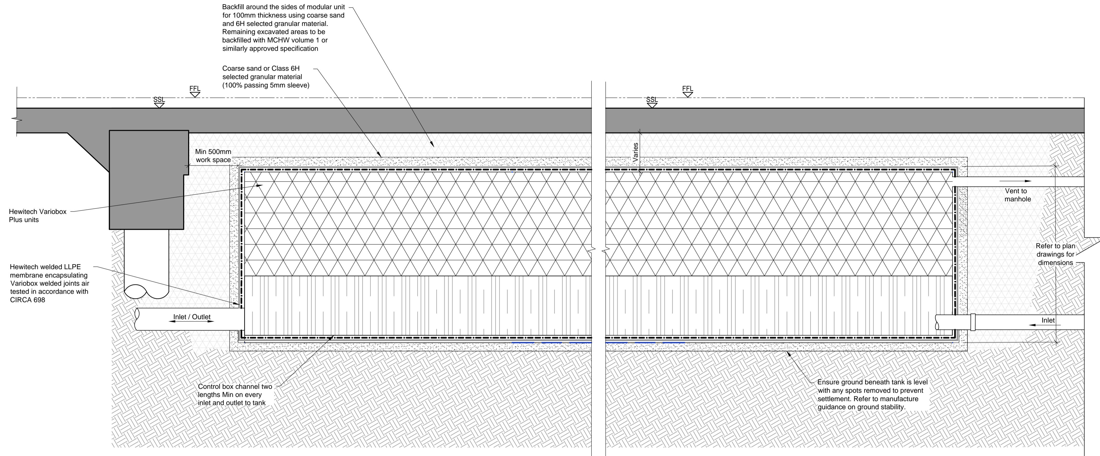
MODULAR ATTENUATION TANK DETAILS - BELOW SLAB (REFER TO HEWITECH SPECIFICATION FOR FULL DETAILS)
