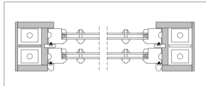
Typical plan view details
