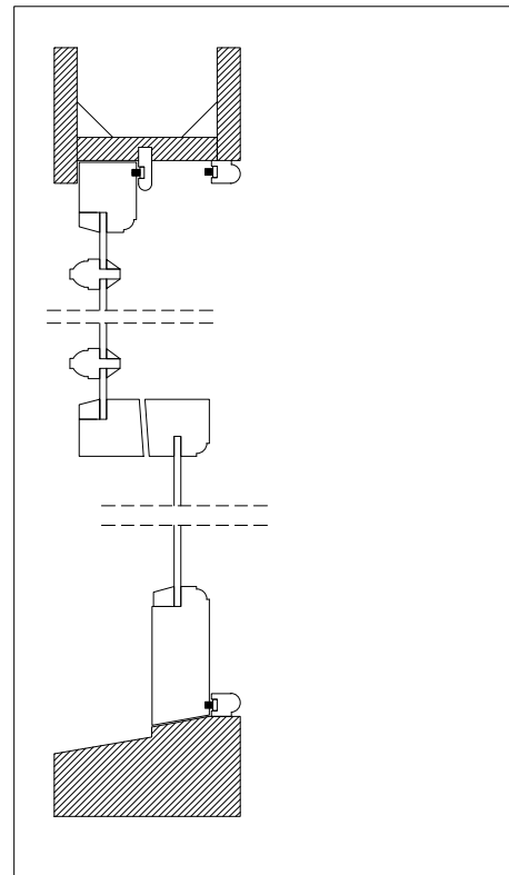
Typical section details
