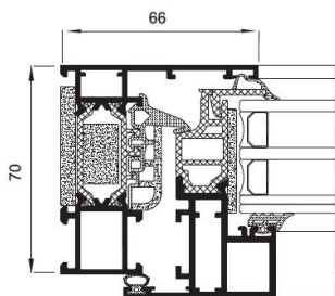
Technical Cross Section
