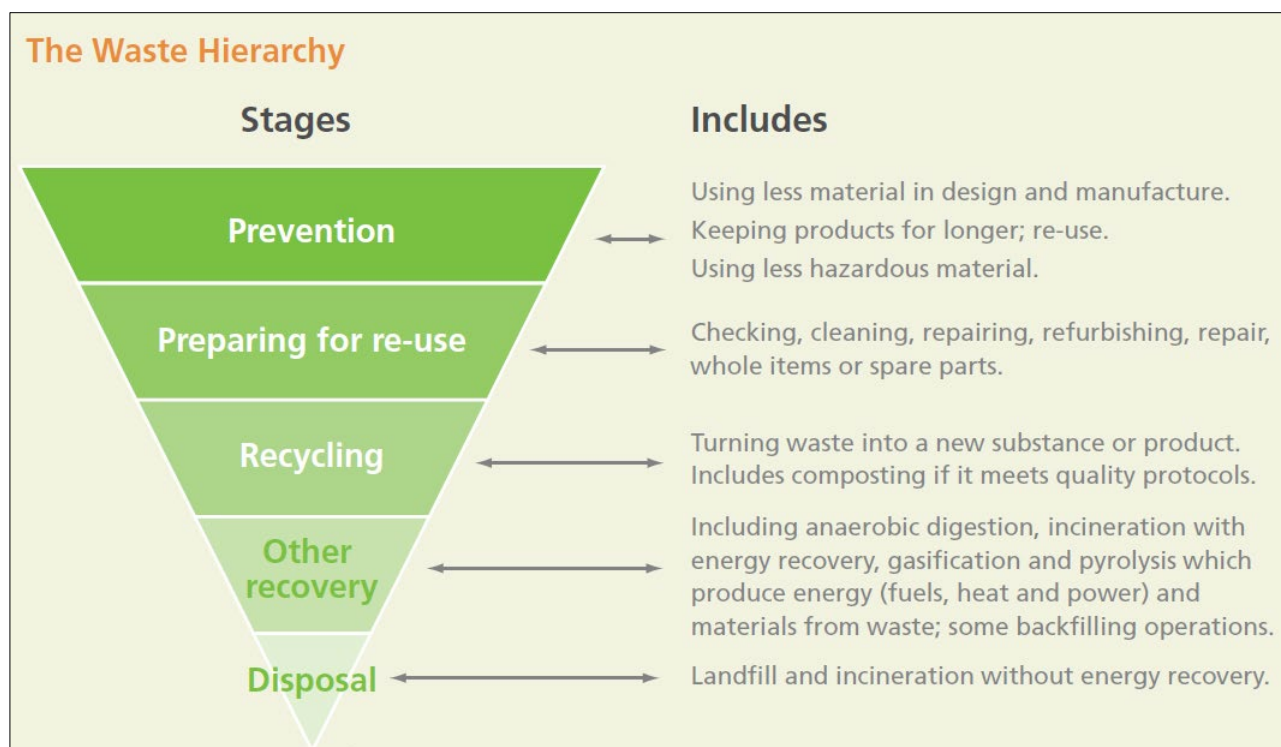
Figure 2.1: Waste Hierarchy
