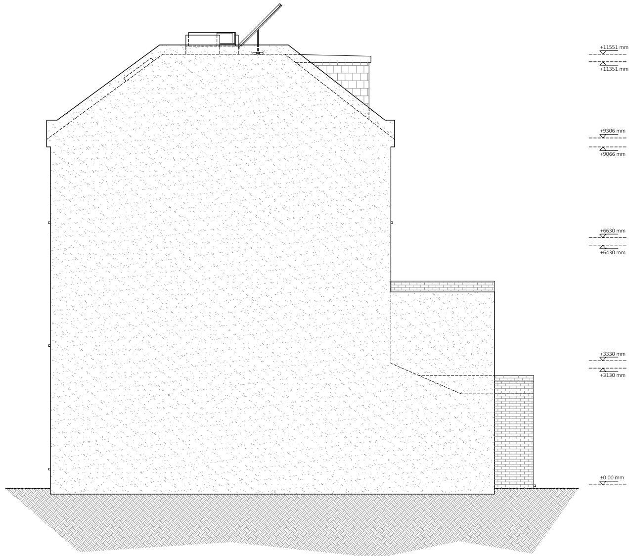
EXISTING EAST SIDE ELEVATION
