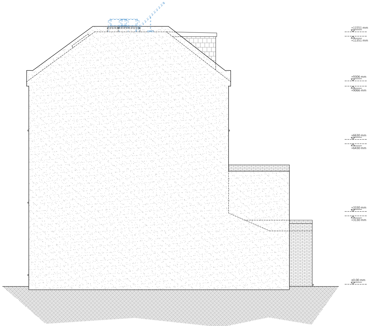
PROPOSED EAST SIDE ELEVATION
