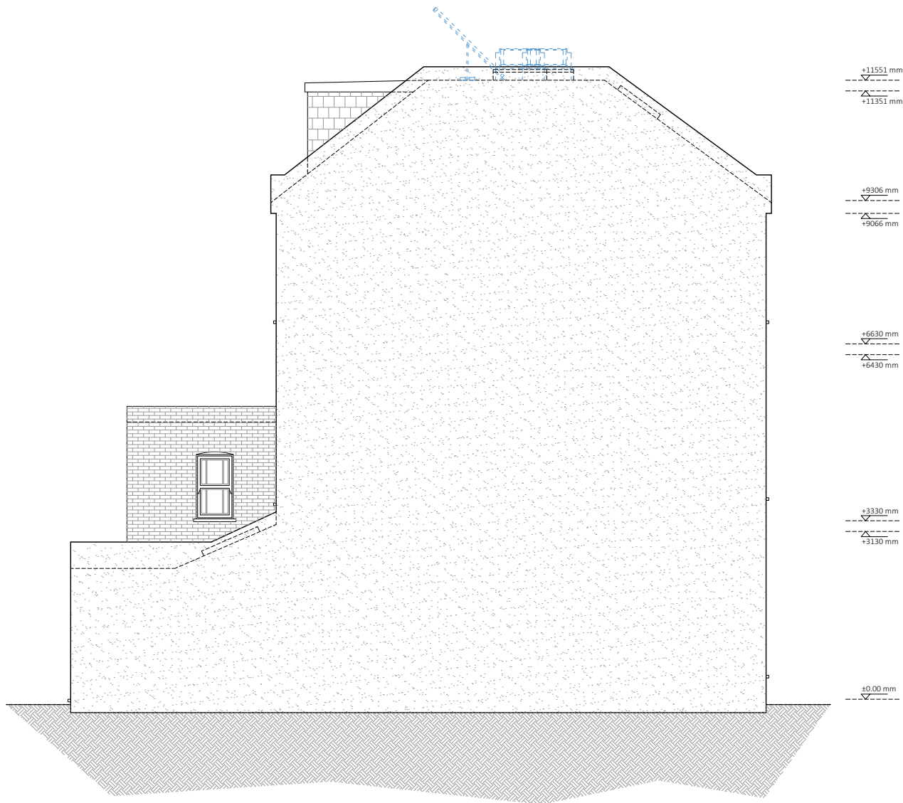
PROPOSED WEST SIDE LEVATION
