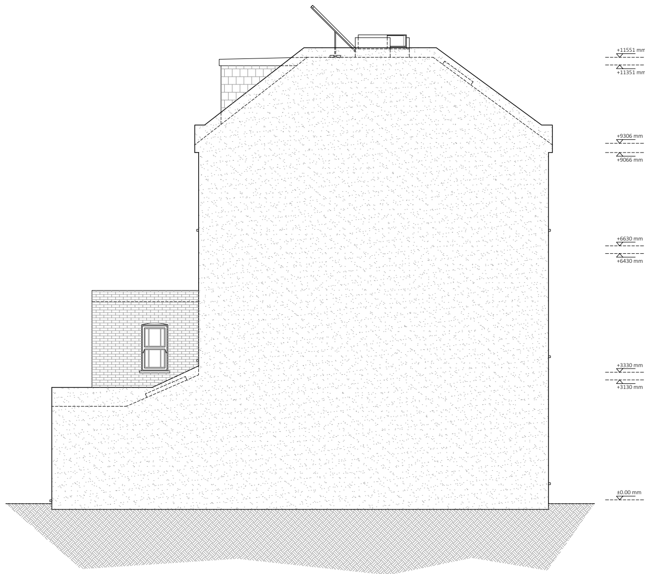
EXISTING WEST SIDE ELEVATION
