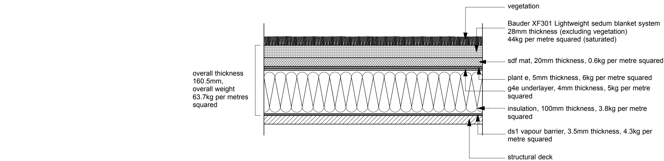
sedum blanket green roof system section detail 1:5
