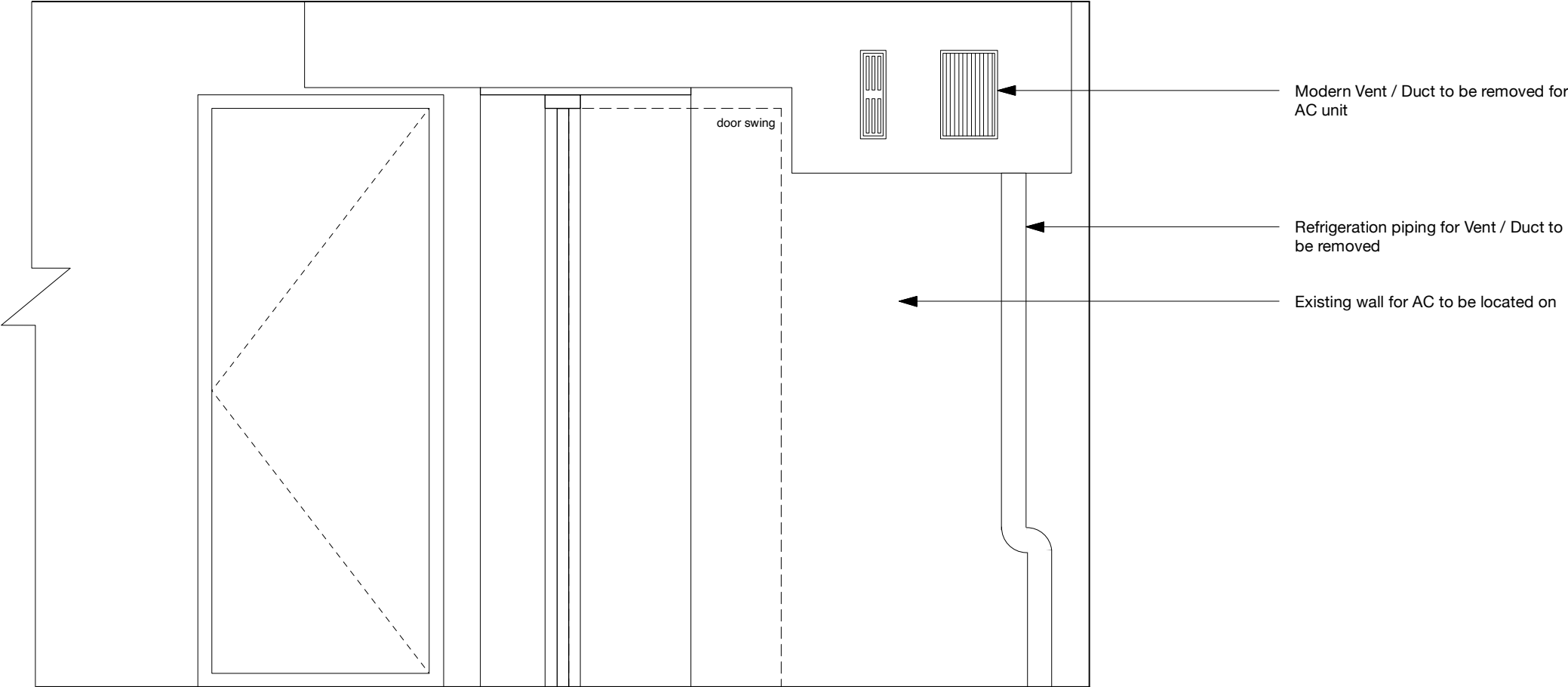
0 0.50 1.00m SCALE 1:20 Section AA
