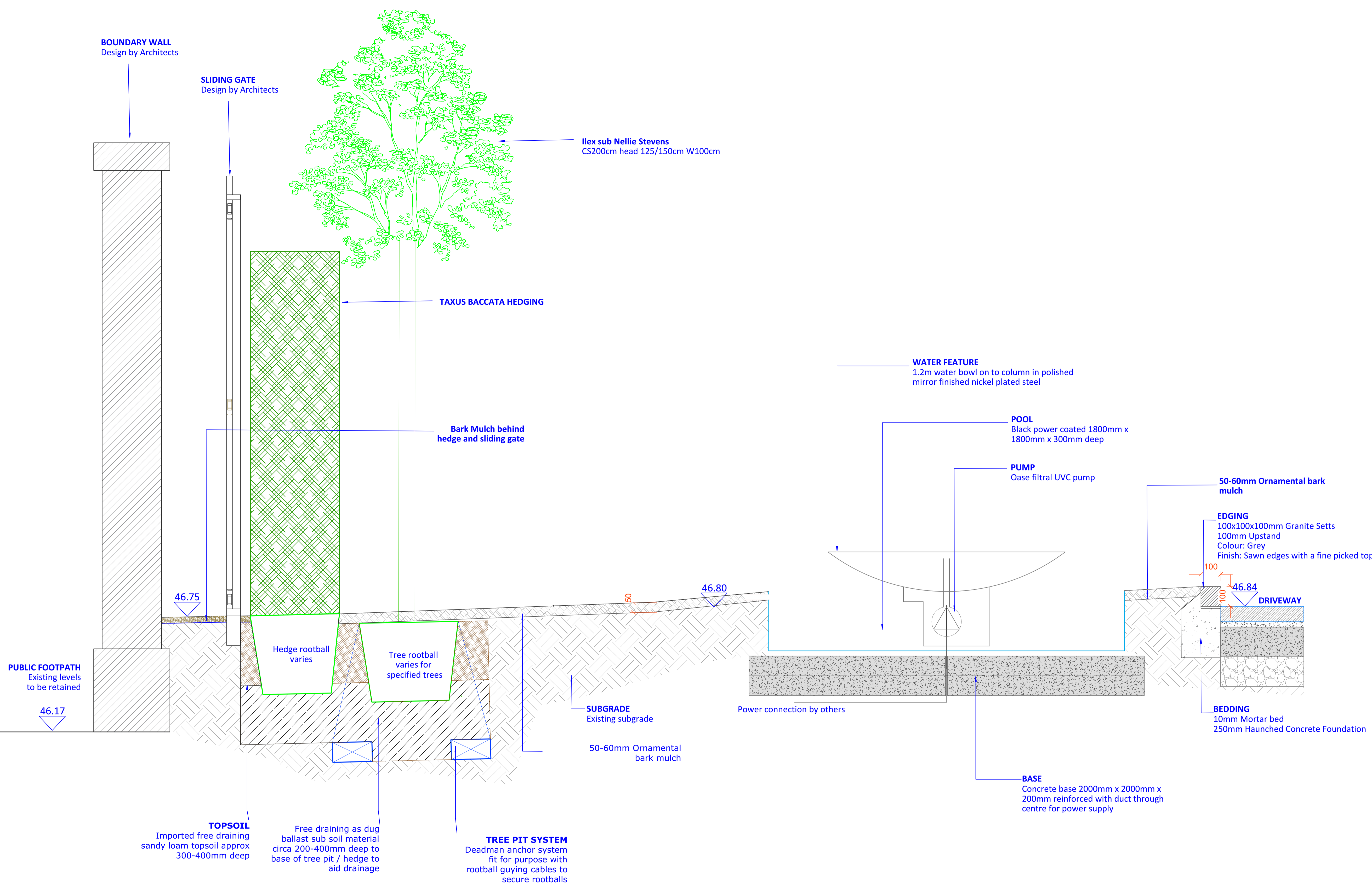
A Detail Section - Front Garden Planting Bed Adjacent to Driveway 1:10@A1
