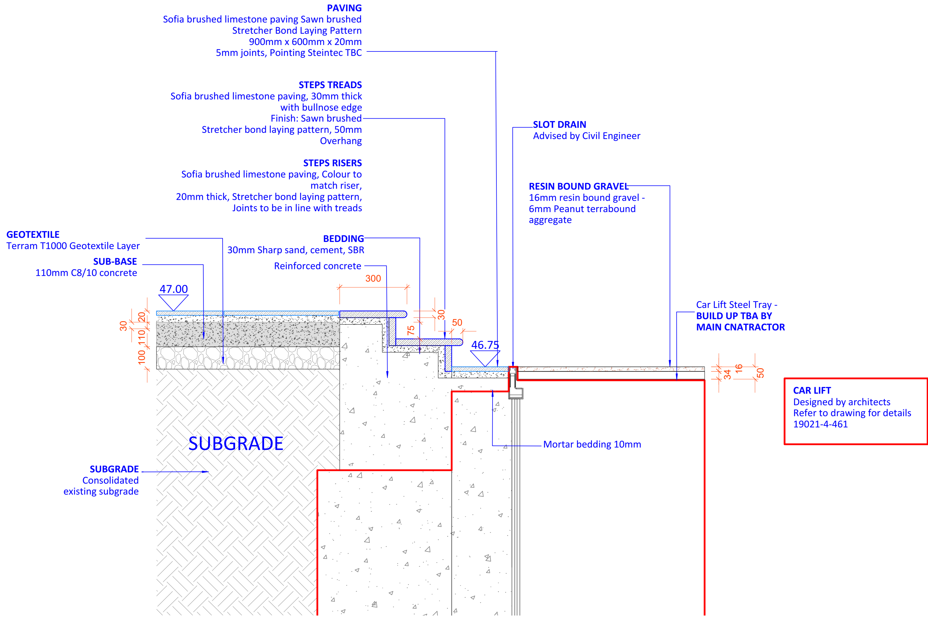
E Detail Section - Front Garden Steps down to Car Lift 1:10@A1
