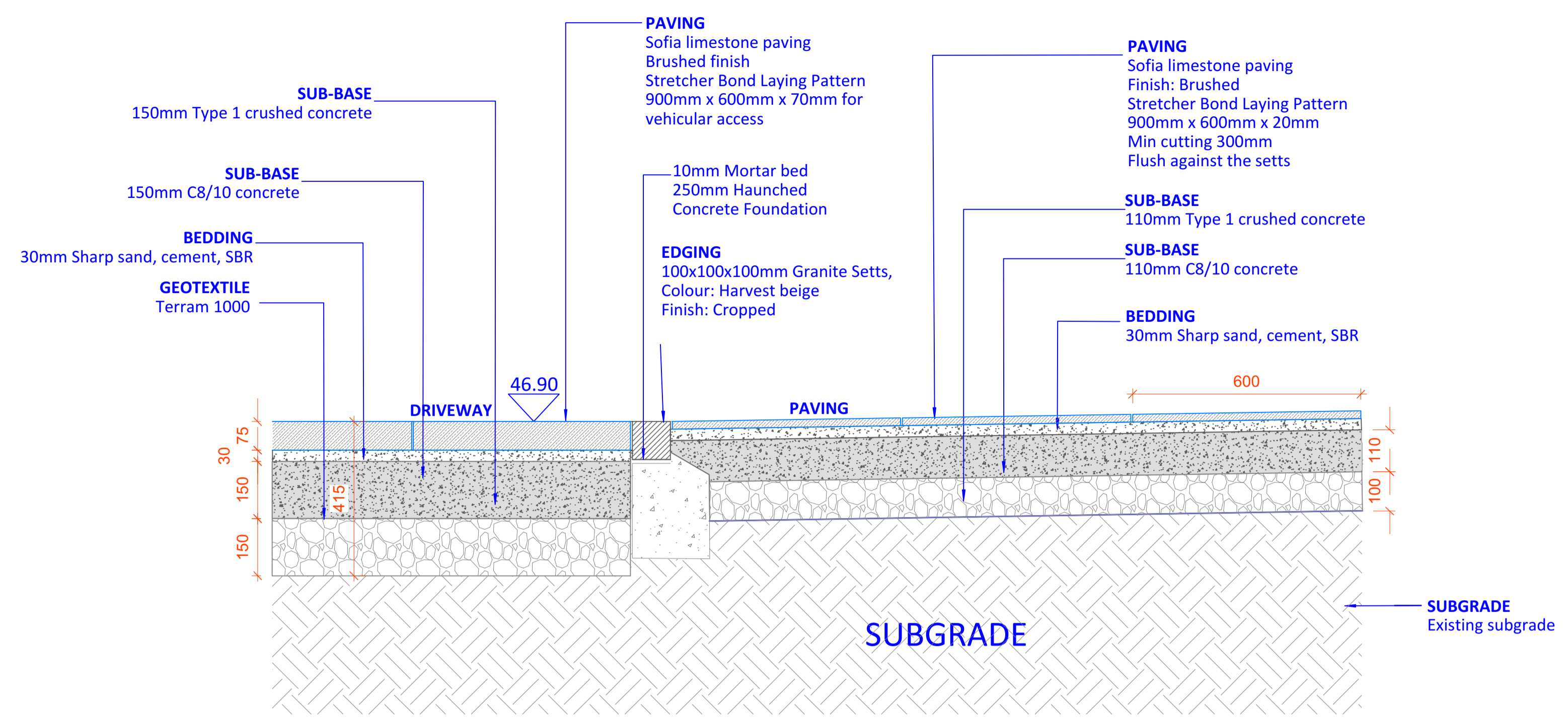
B Detail Section - Front Garden Driveway to Main Entrance Paving 1:10@A1
