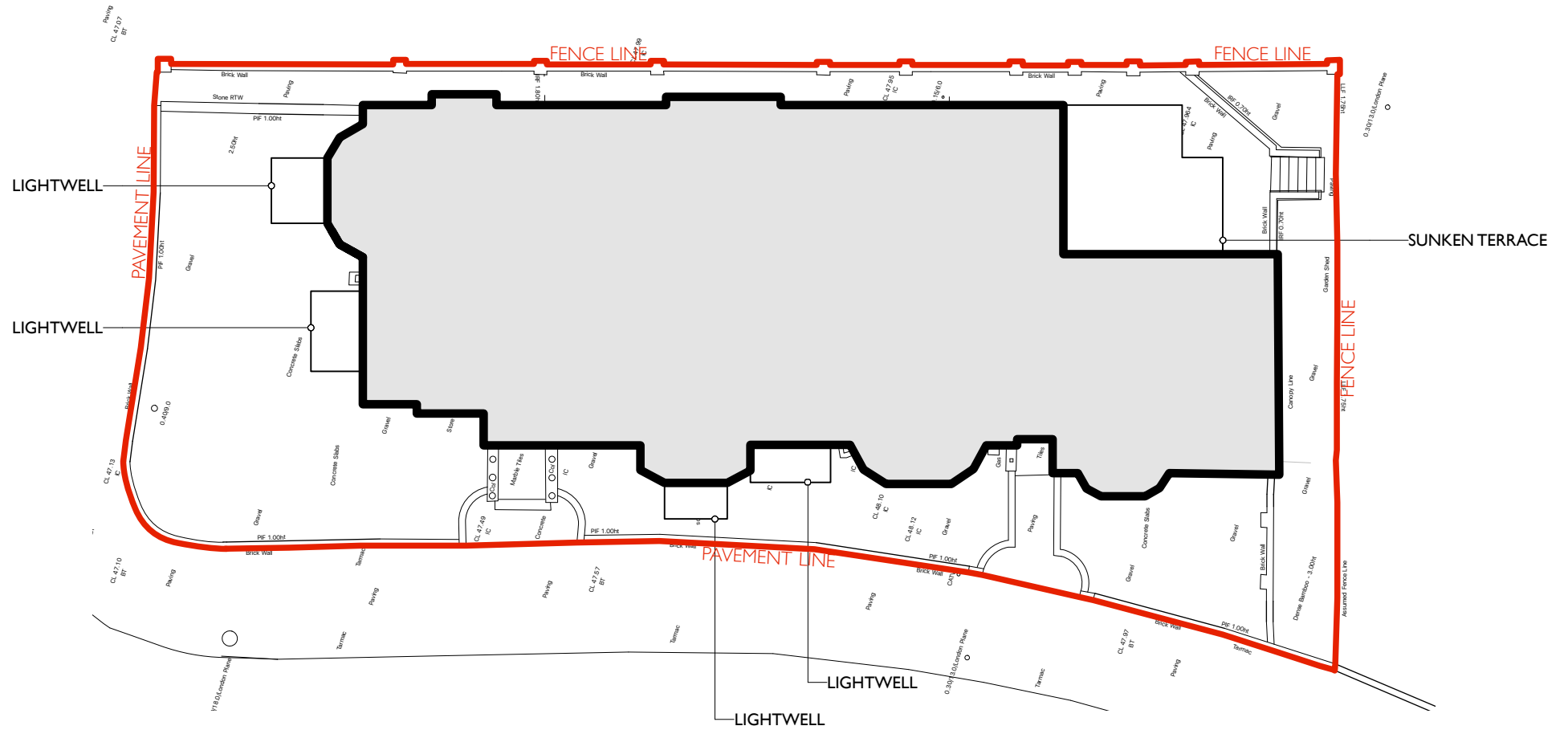
BLOCK PLAN
