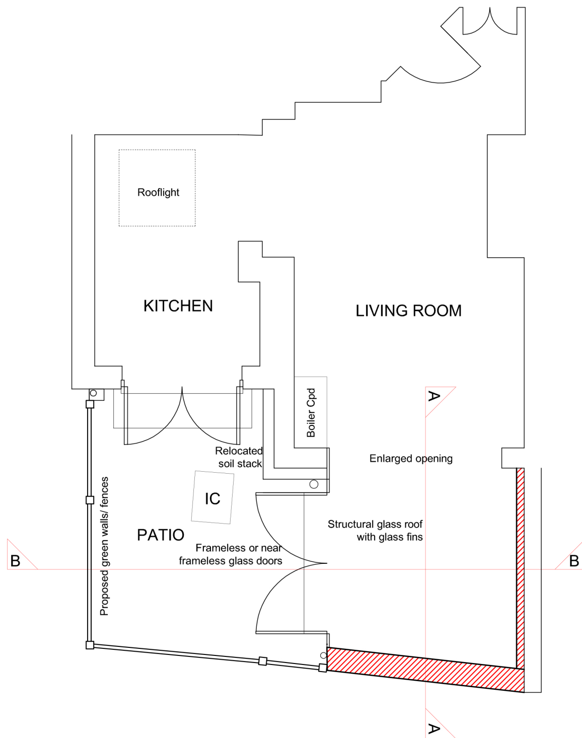
Proposed Extract Ground Floor Plan
