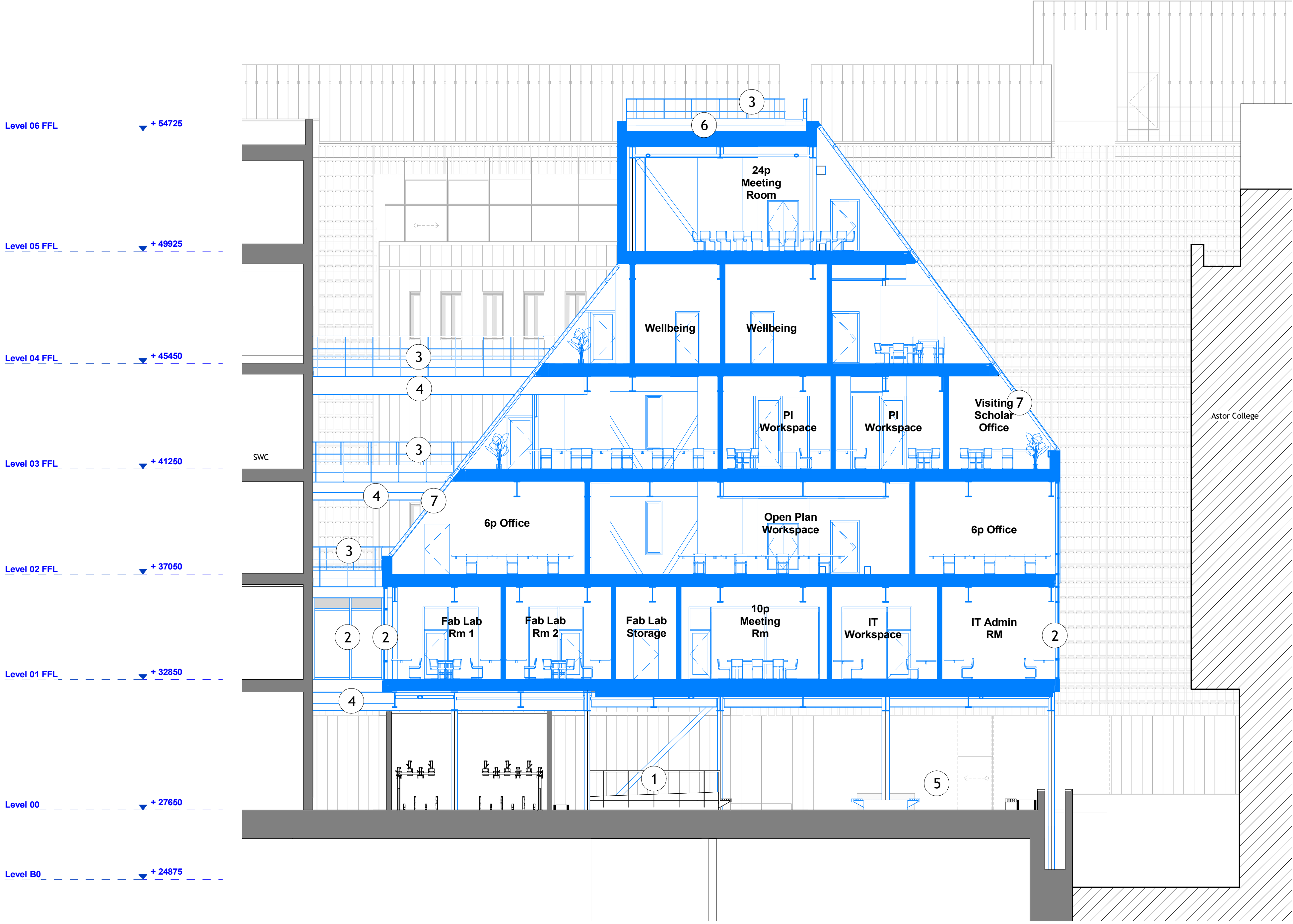
1 E-W GA Section Looking North 1 : 100
