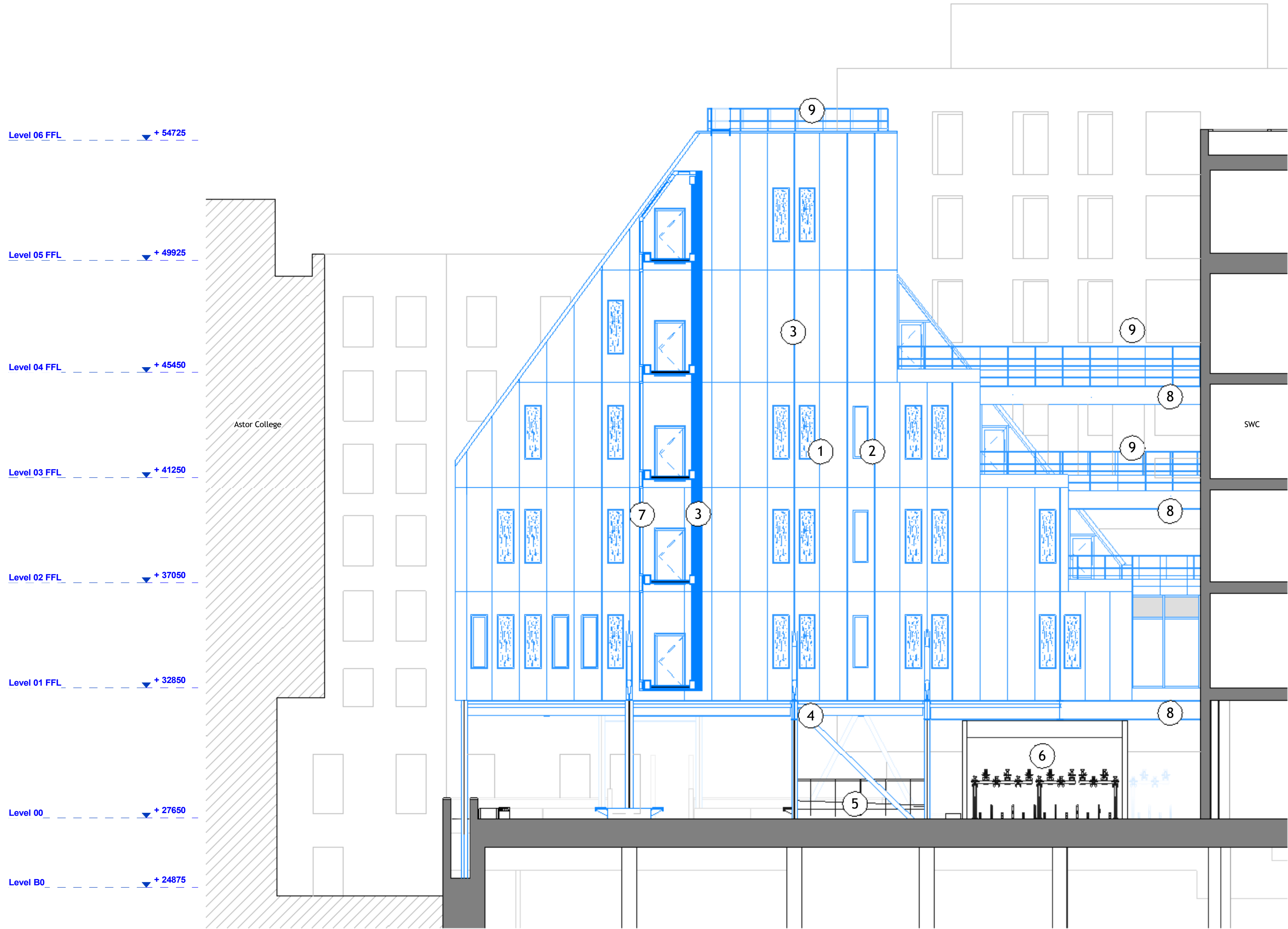
1 Proposed North GA Elevation 1 : 100
