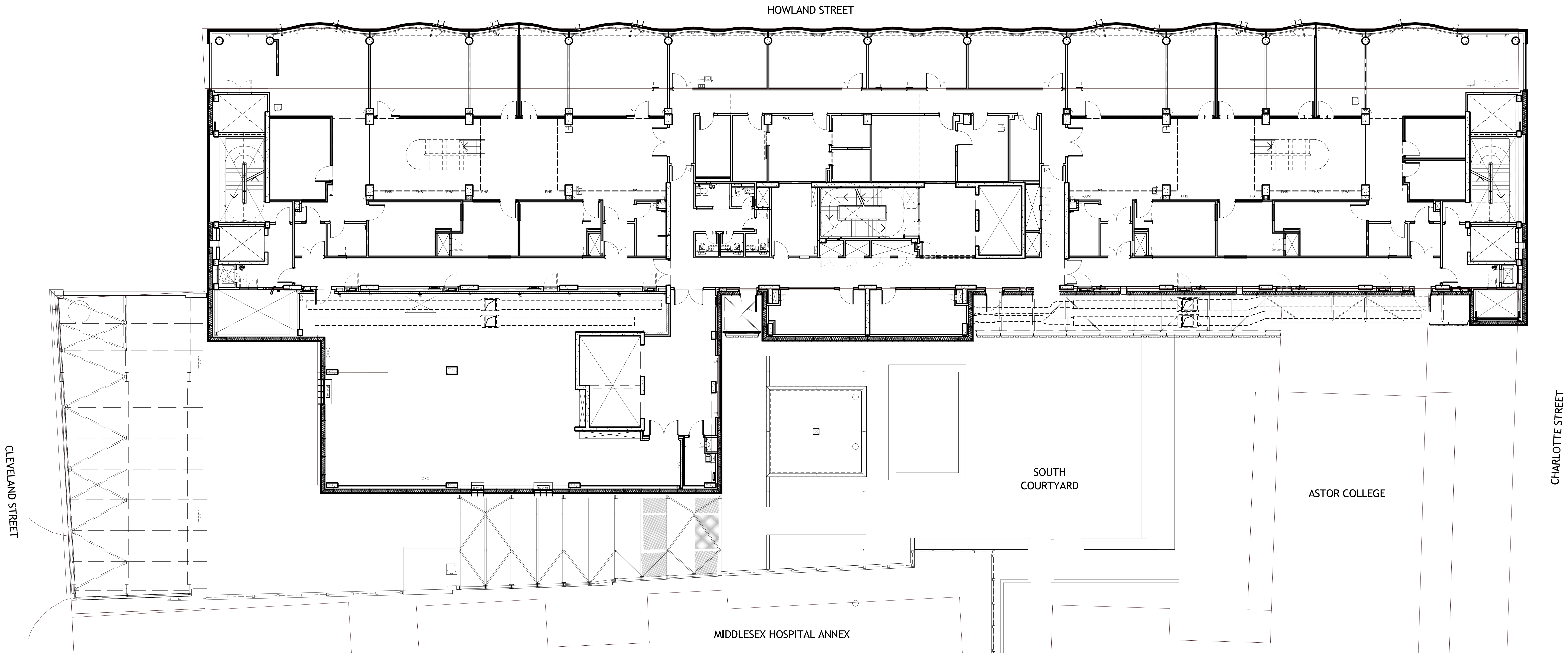
1 Existing First Floor GA Plan 1 : 100
