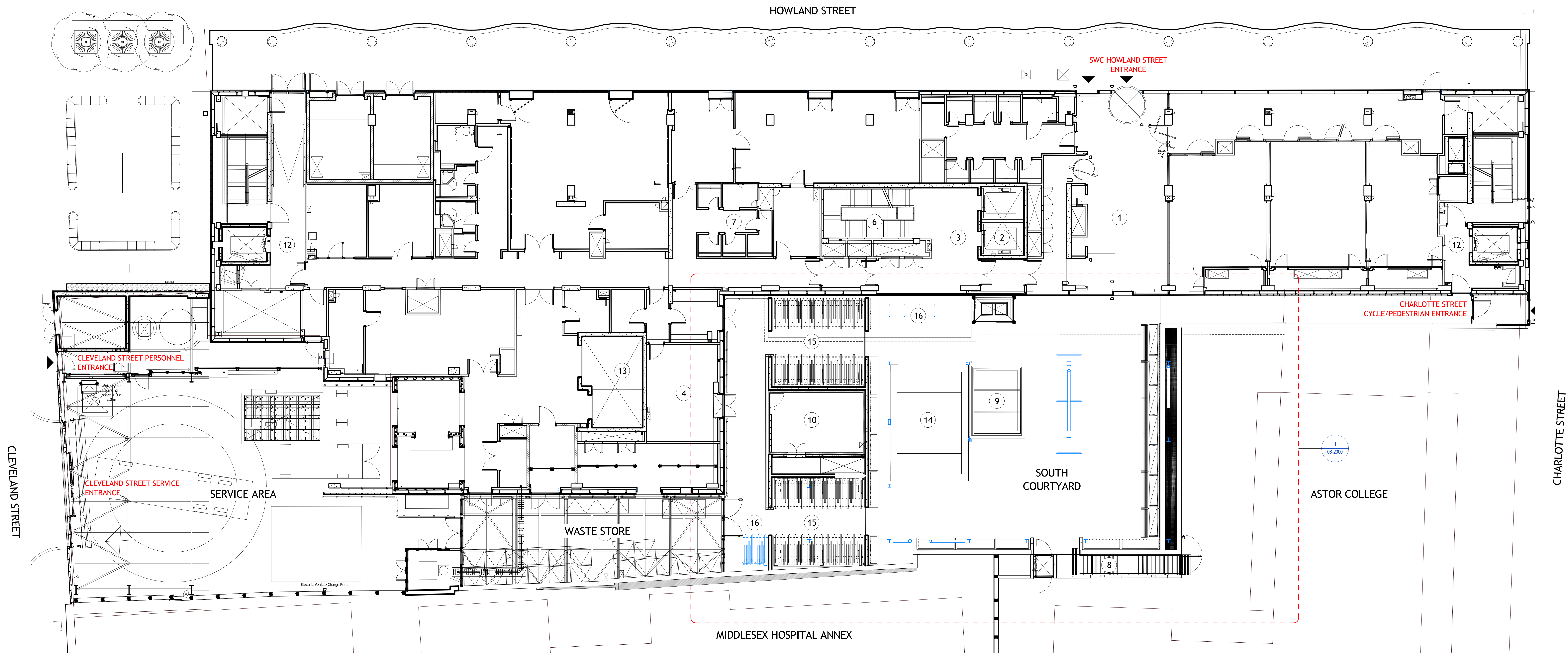
1 Proposed Ground Floor GA Plan 1 : 100
