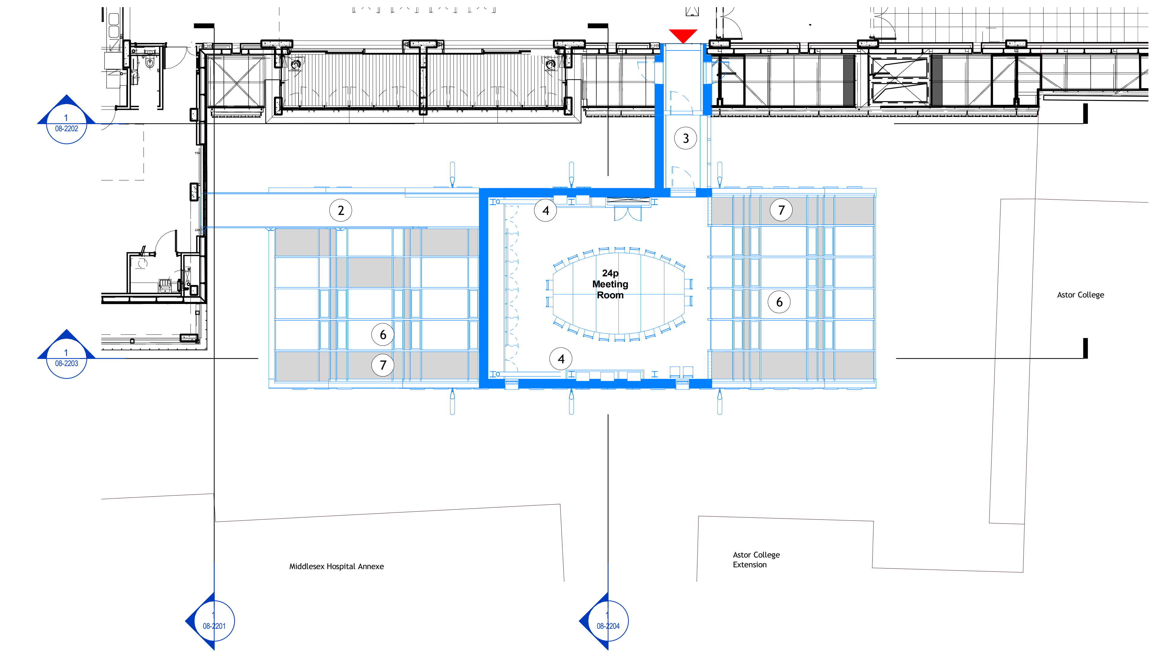
1 Proposed 5th Quad Level 05 GA Plan 1 : 100
