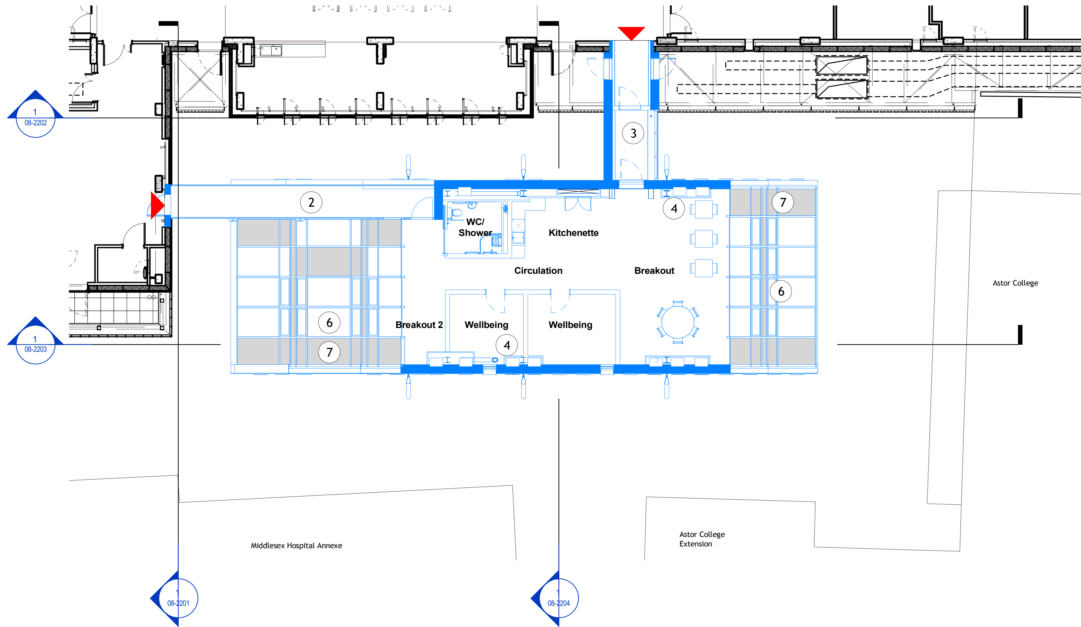
1 Proposed 5th Quad Level 04 GA Plan 1 : 100
