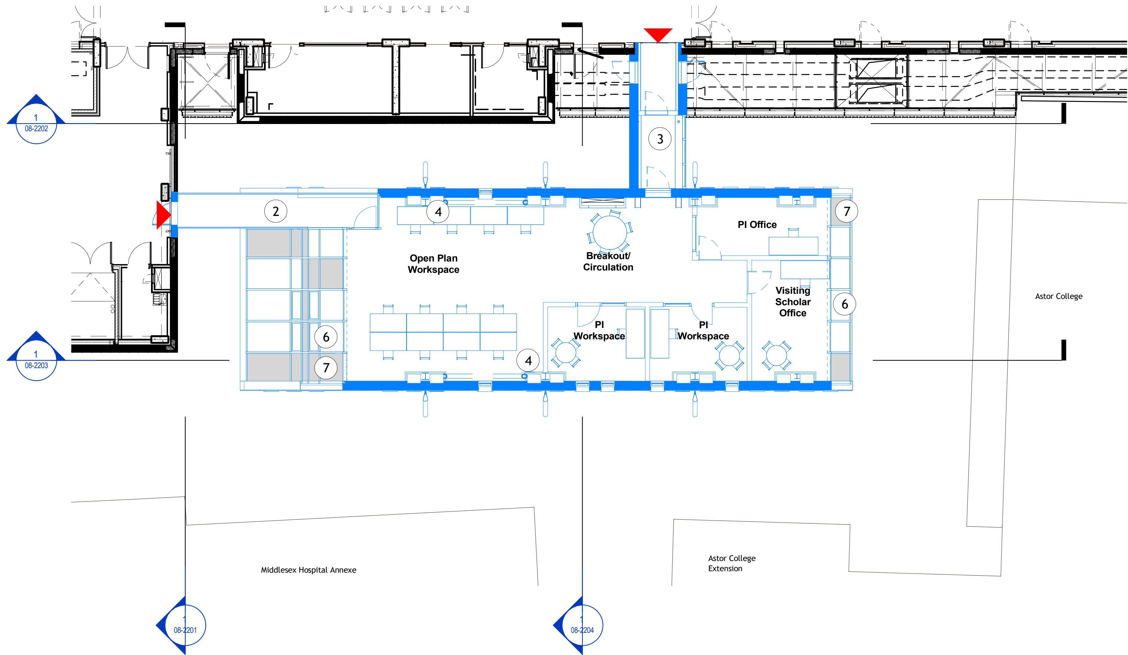
1 Proposed 5th Quad Level 03 GA Plan 1 : 100
