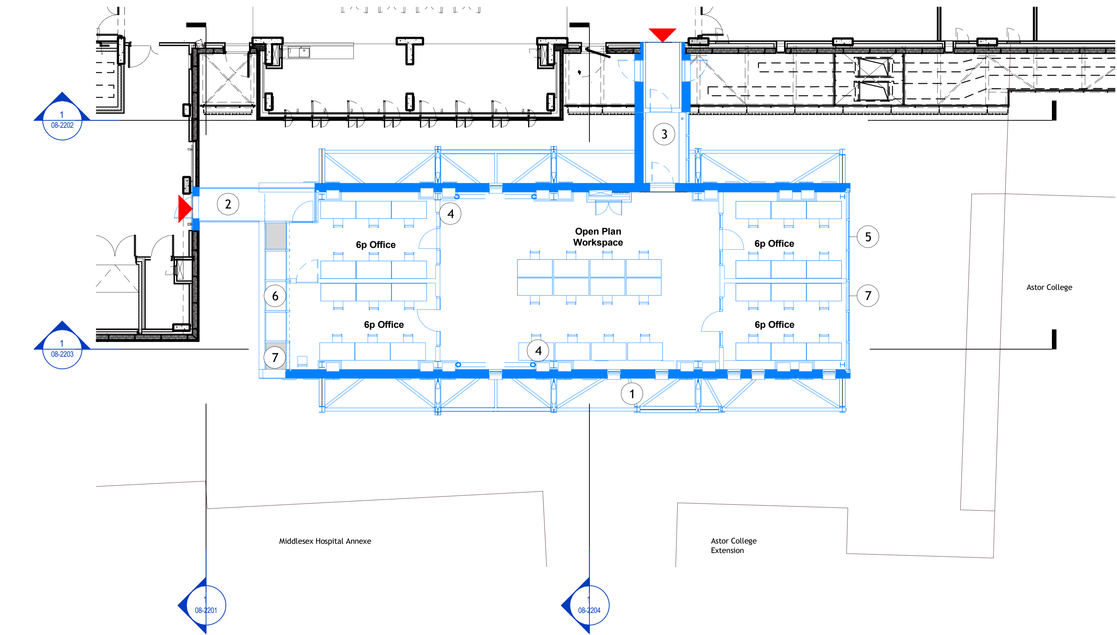
1 Proposed 5th Quad Level 02 GA Plan 1 : 100
