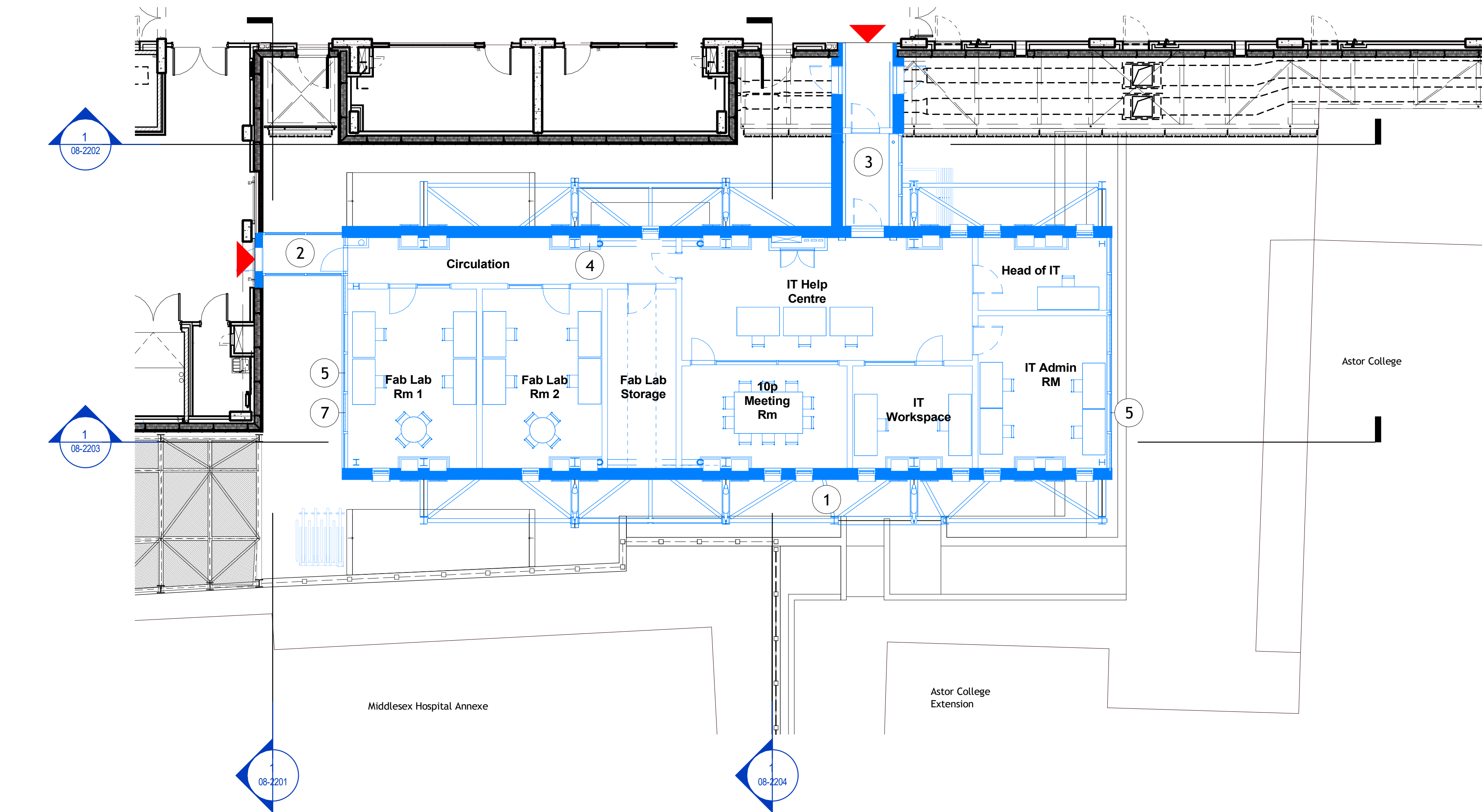
1 Proposed 5th Quad Level 01 GA Plan 1 : 100
