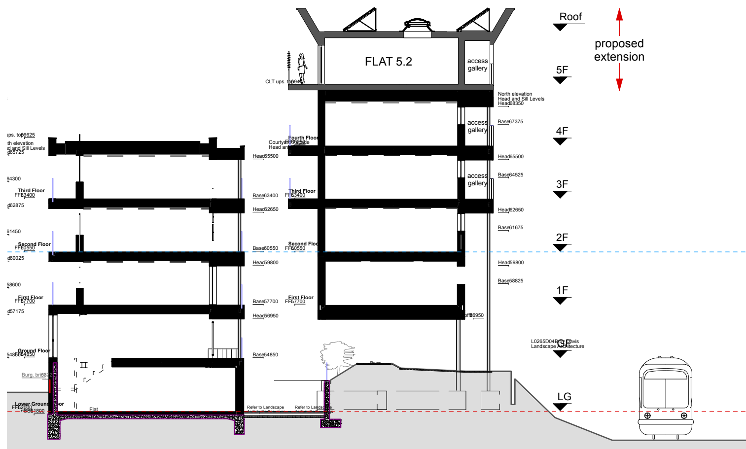
SECTION F-F'
