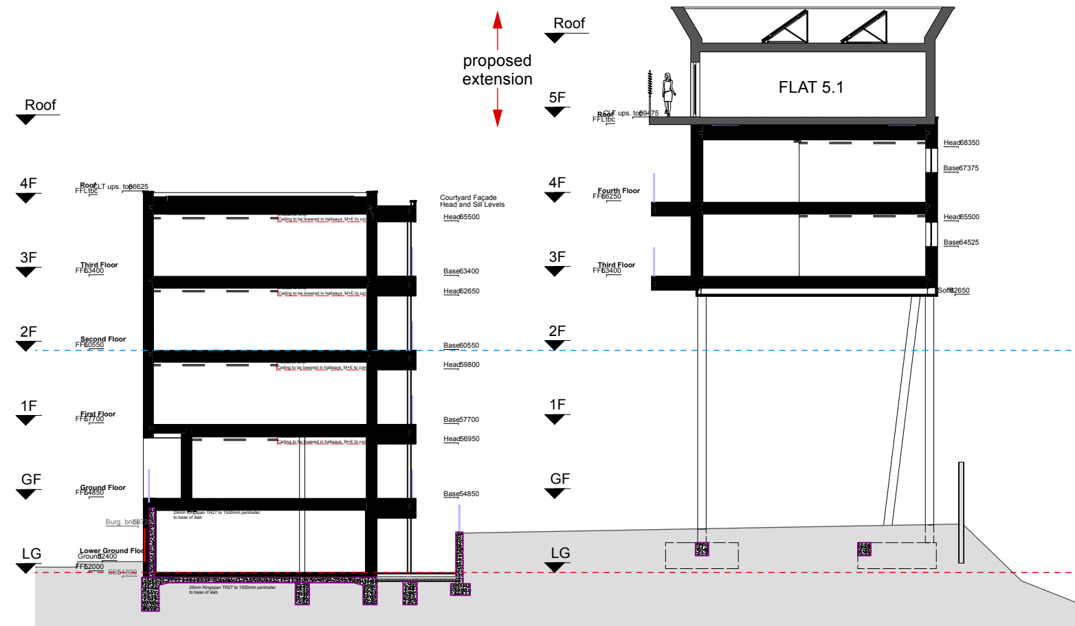
SECTION G-G'
