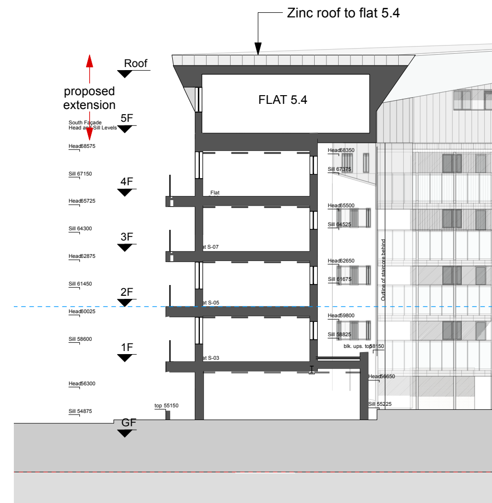
SECTION CC
