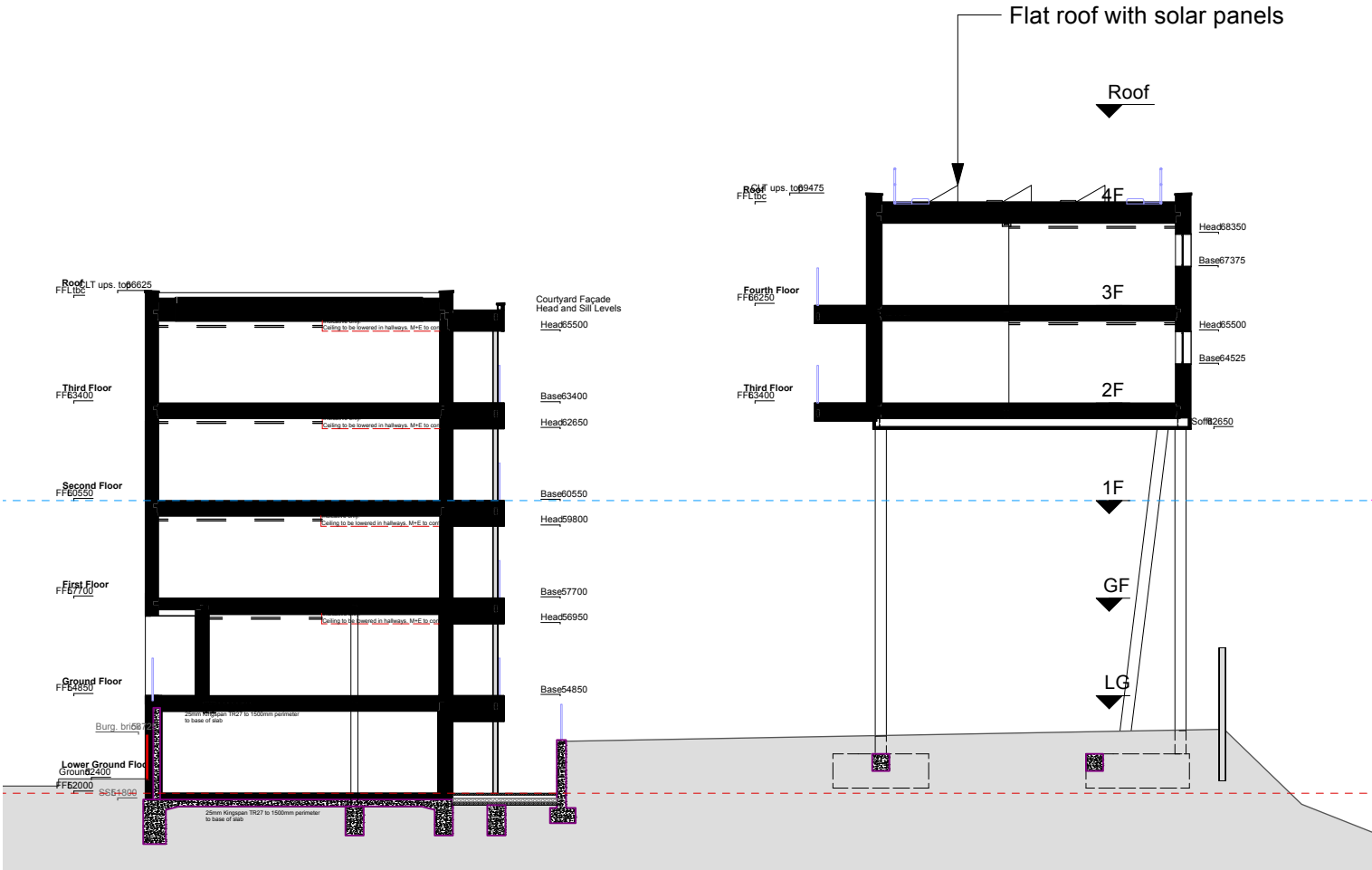
SECTION G-G'
