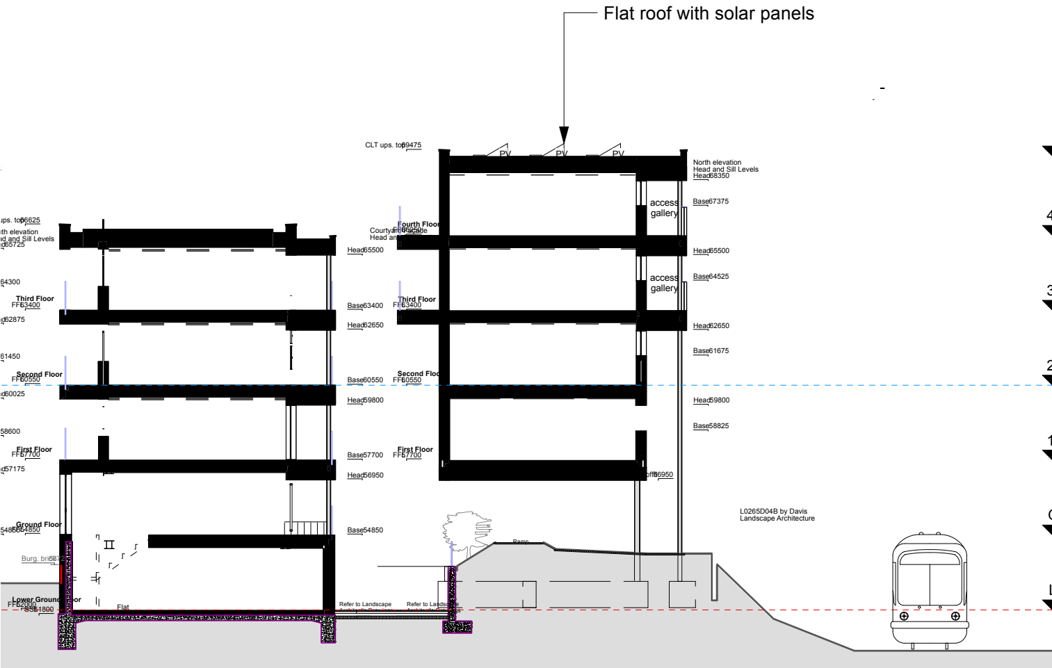
SECTION F-F'
