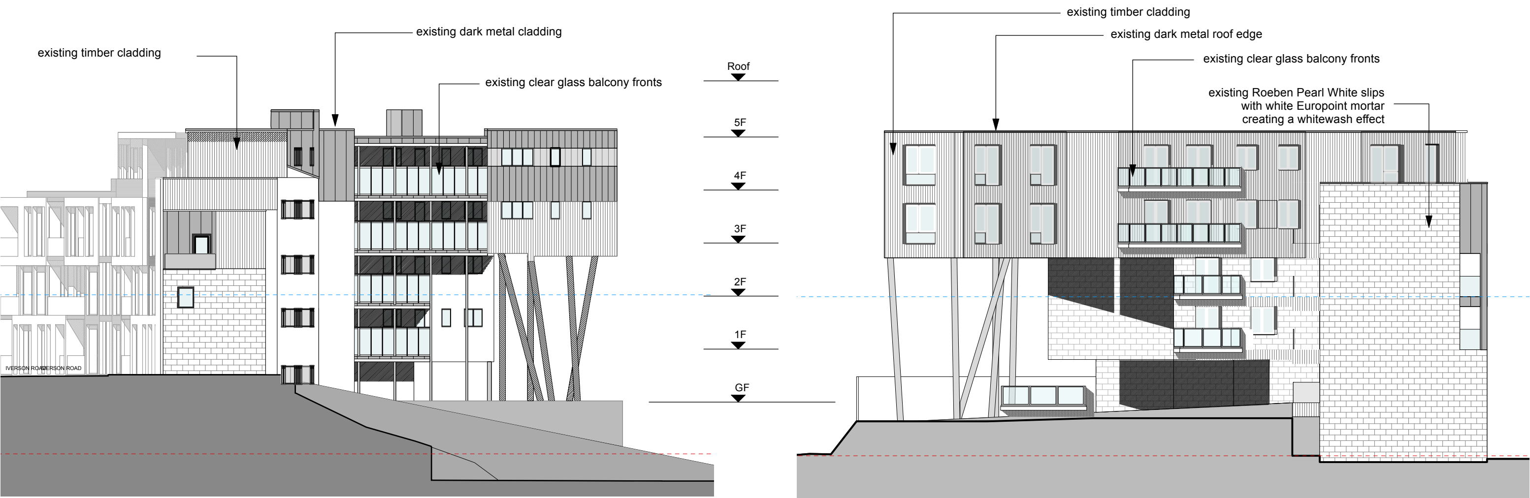
EAST ELEVATION
