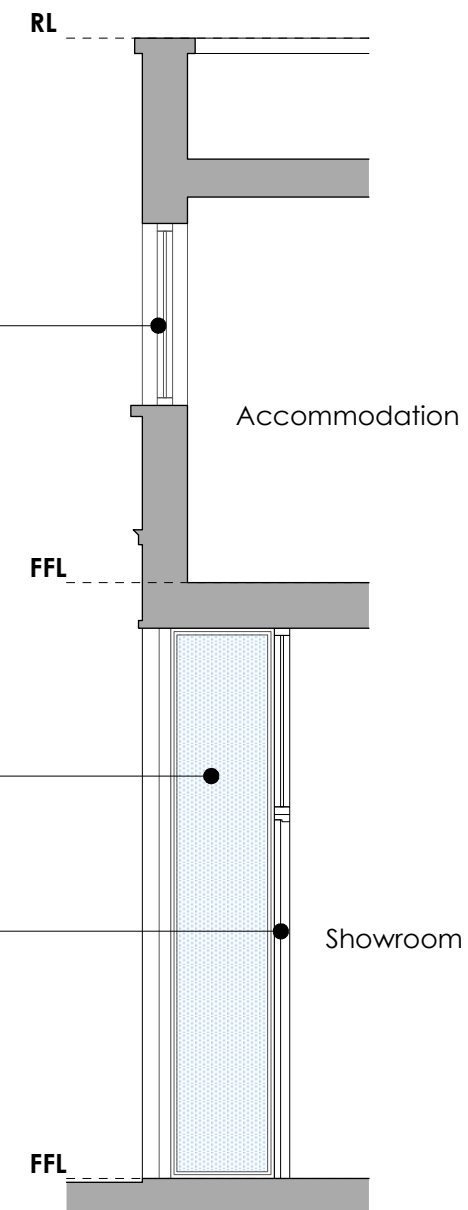
2 Proposed Front / Street Section scale: 1:50 @ A3
