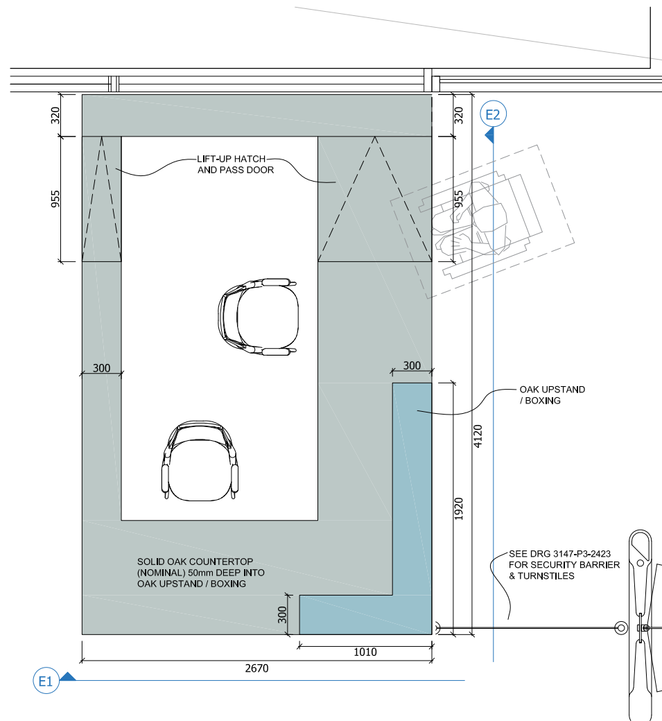
3 L4 RECEPTION JOINERY - HIGH LEVEL PLAN 1:20
