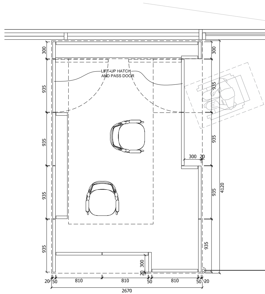
2 L4 RECEPTION JOINERY - LOW LEVEL PLAN 1:20
