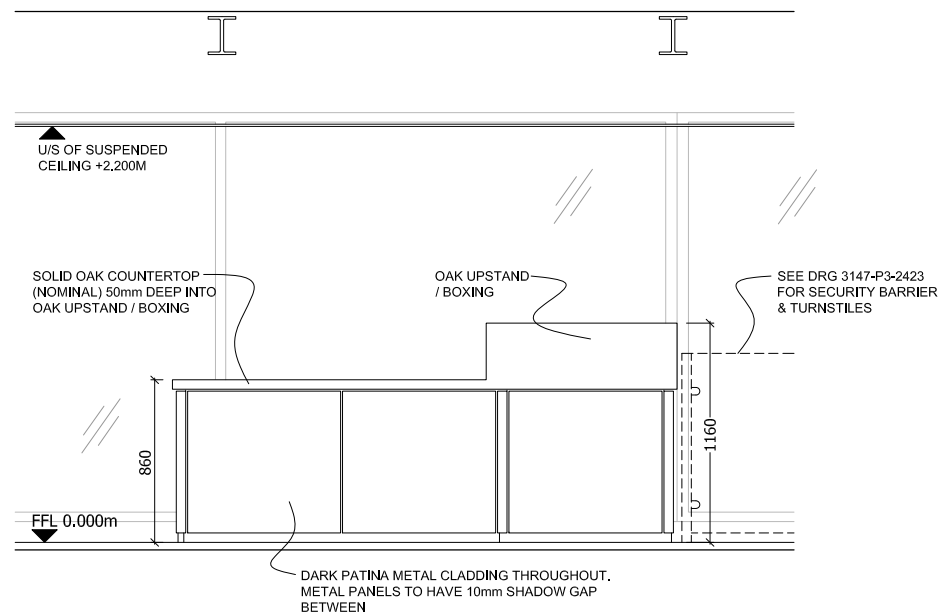
E1 L4 RECEPTION JOINERY ELEVATION 1 1:20
