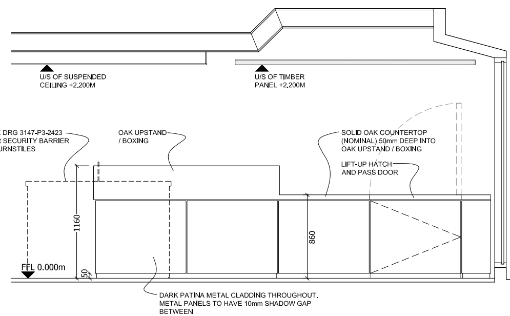
E2 L4 RECEPTION JOINERY ELEVATION 1 1:20
