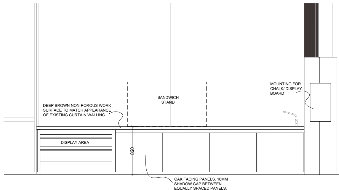
E2 CAFE JOINERY ELEVATION 1:20
