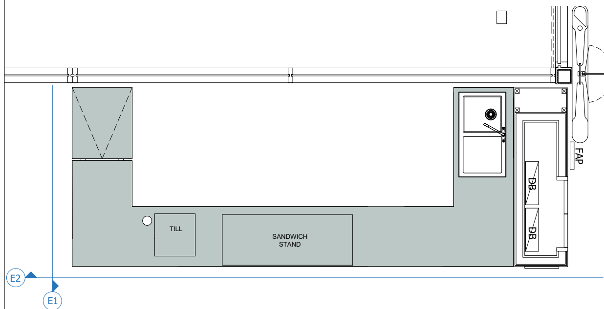
1 CAFE JOINERY - HIGH LEVEL PLAN 1:20
