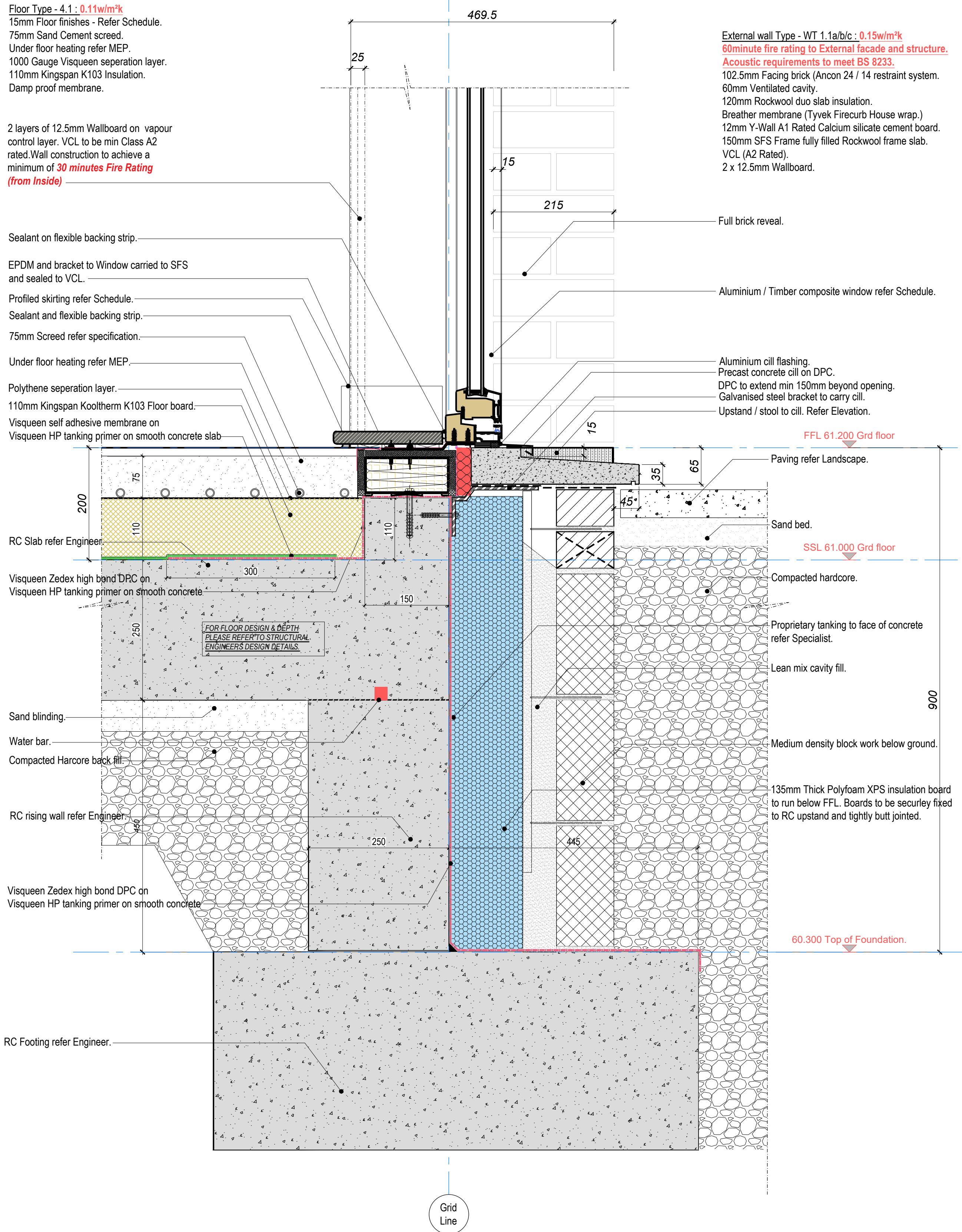
2- GROUND FLOOR FLOOR / WALL JUNCTION -BLOCK A. Scale 1:5
