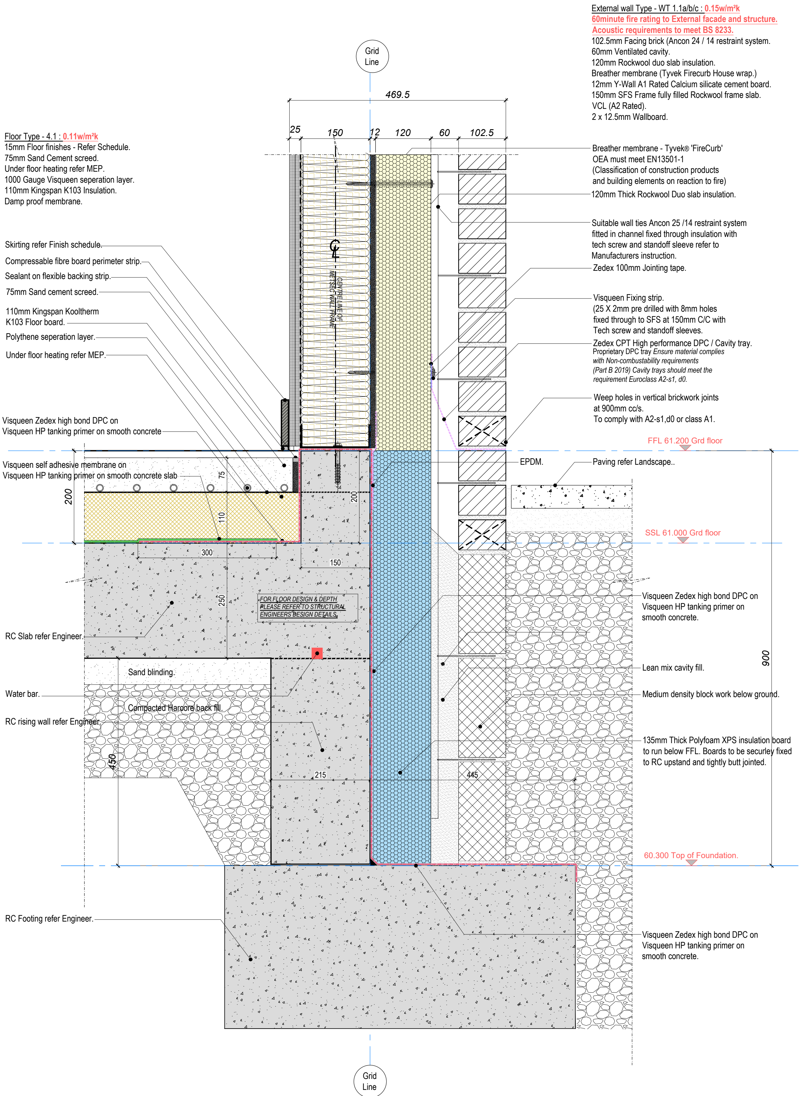
1- GROUND FLOOR FLOOR / WALL JUNCTION -BLOCK A. Scale 1:5
